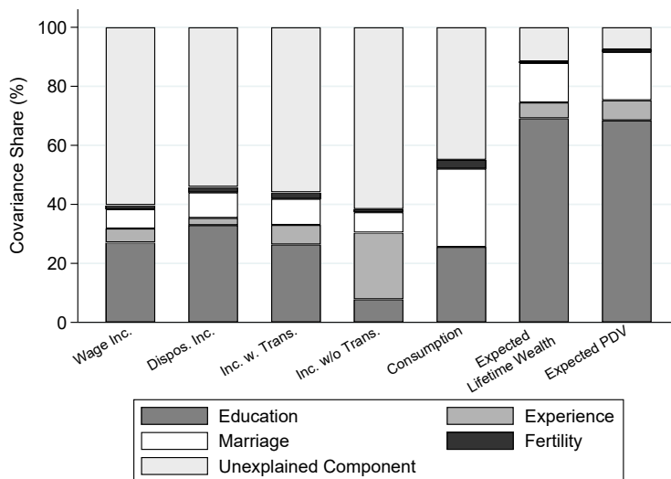
(a) Covariance Share
