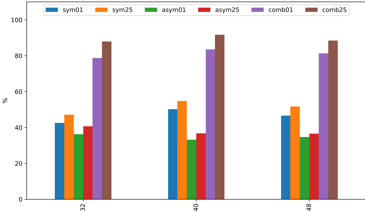
Figure A.18: Weight of beliefs on equilibrium strategies in Supergame 1 vs. Supergame 25 (split by R )
