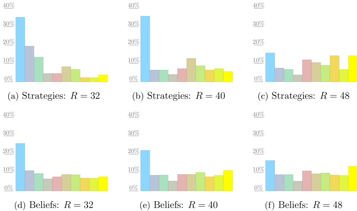
Figure A.20: Strategies & average beliefs in Supergame 1 (replicates Figure 3)
