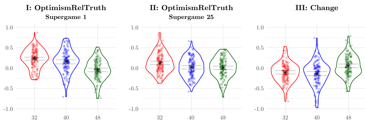
Figure A.16: Evolution of OptimismRelTruth at the session level: Violin plots
