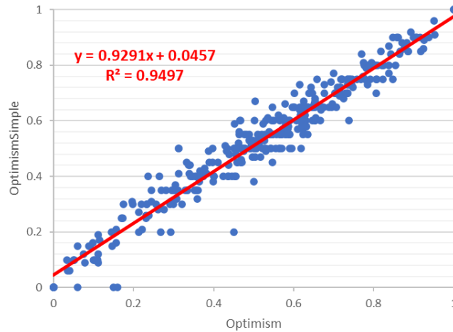
Figure A.13: Scatterplot of OptimismSimple vs. Optimism in Supergame 1
