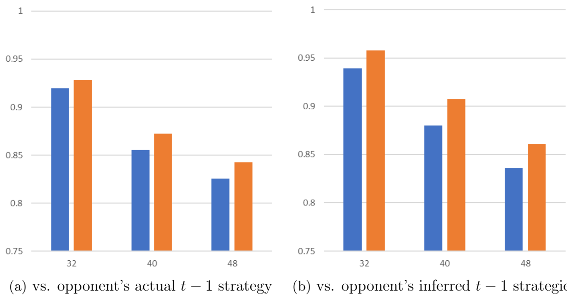
Figure A.19: Payoff of revised strategy at t (orange) and original strategy at t - 1 (blue), playing against opponent's t - 1 strategy (as proportion of payoff from best-response)
