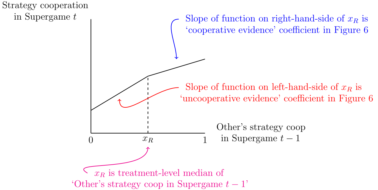
Figure 7: Understanding the coefficients from Figure 6
