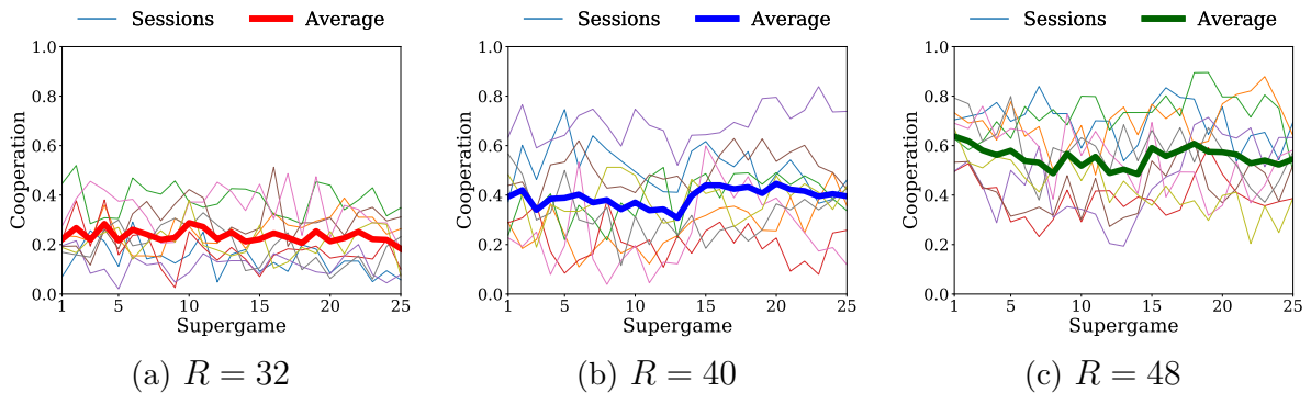
Figure 5: Evolution of cooperation across supergames
