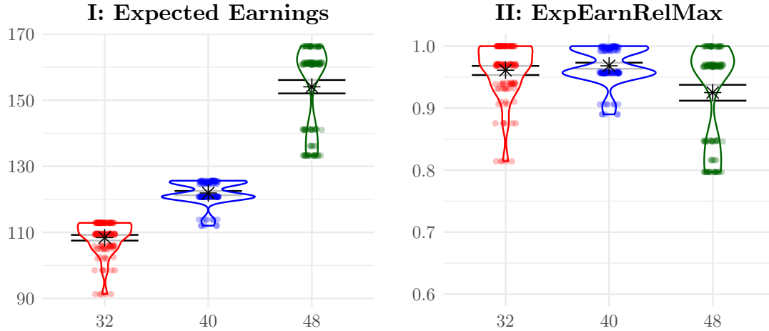
Figure A.15: Earnings in Supergame 1: Violin plots
