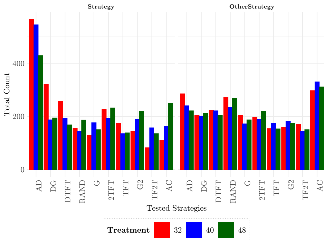
Figure A.24: Number of times each strategy was tested during the training phase
