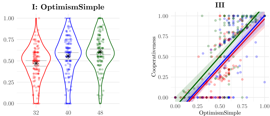
Figure A.14: Panels I and III of Figure 4, using OptimismSimple instead of Optimism
