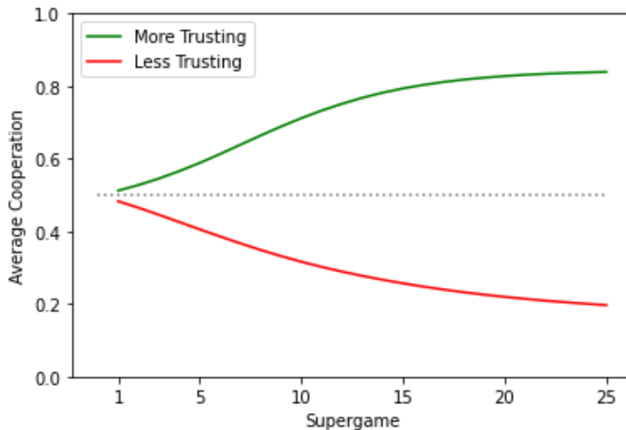
Figure A.23: Simulated dynamics of cooperation in more trusting and less trusting sessions
