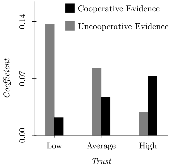
Figure 6: Effect of opponent’s strategy cooperation in Supergame t - 1 on strategy cooperation in Supergame t
