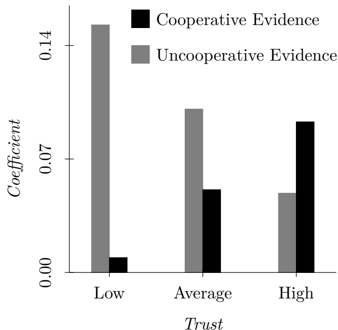
Figure A.22: Effect of opponent's strategy cooperation in Supergame t - 1 on strategy cooperation in Supergame t (robustness)
