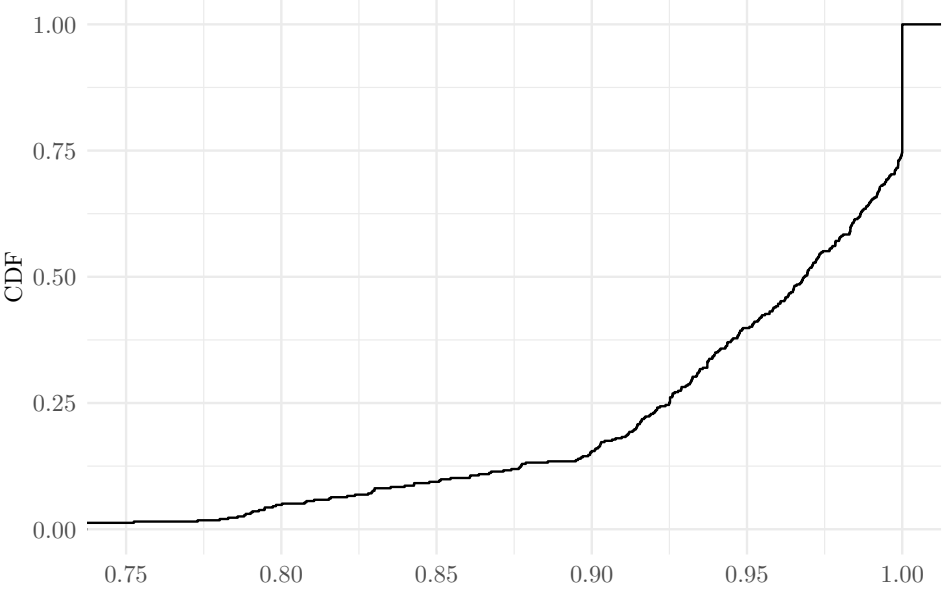
Figure A.25: CDF of payoffs relative to best responding to beliefs in Supergame 1
