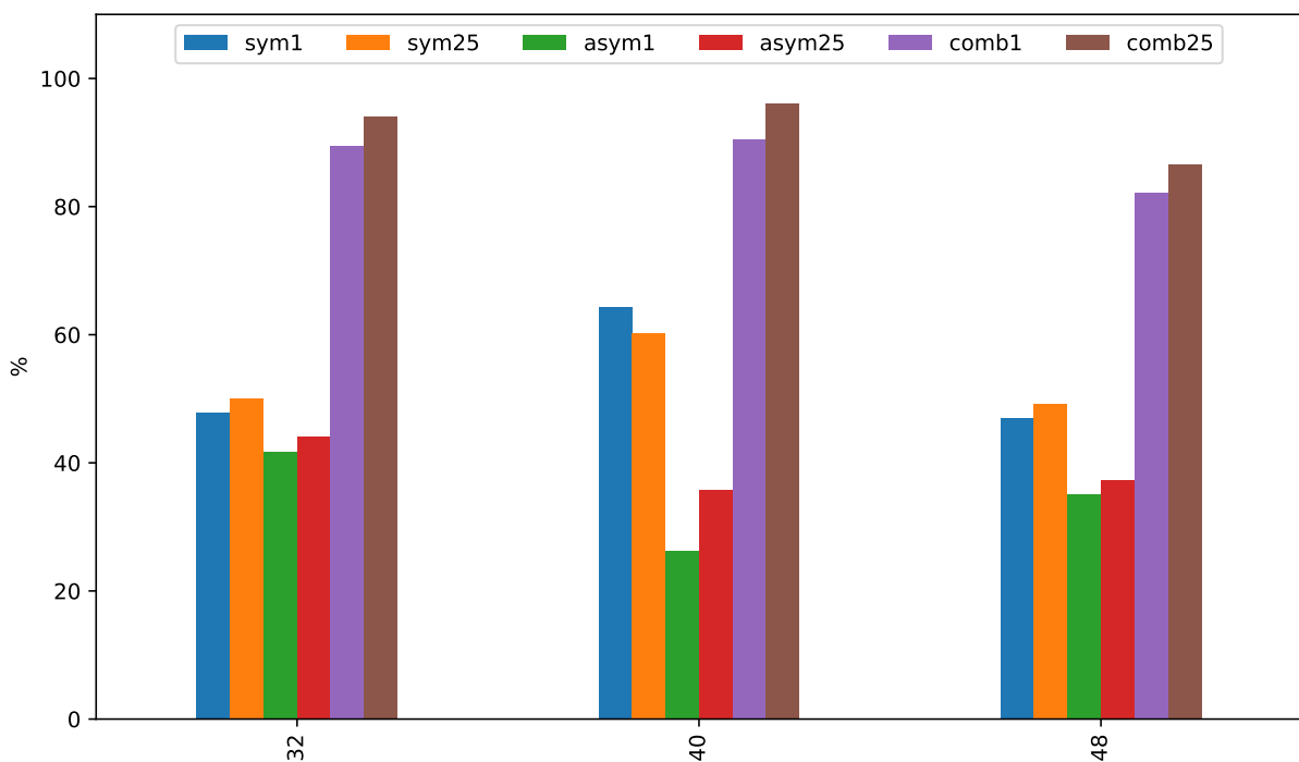
Figure A.17: Equilibrium strategies as proportion of chosen strategies in Supergame 1 vs. Supergame 25 (split by R )
