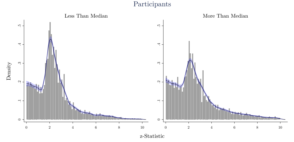
Figure 12: z-Statistics by Sample Size
