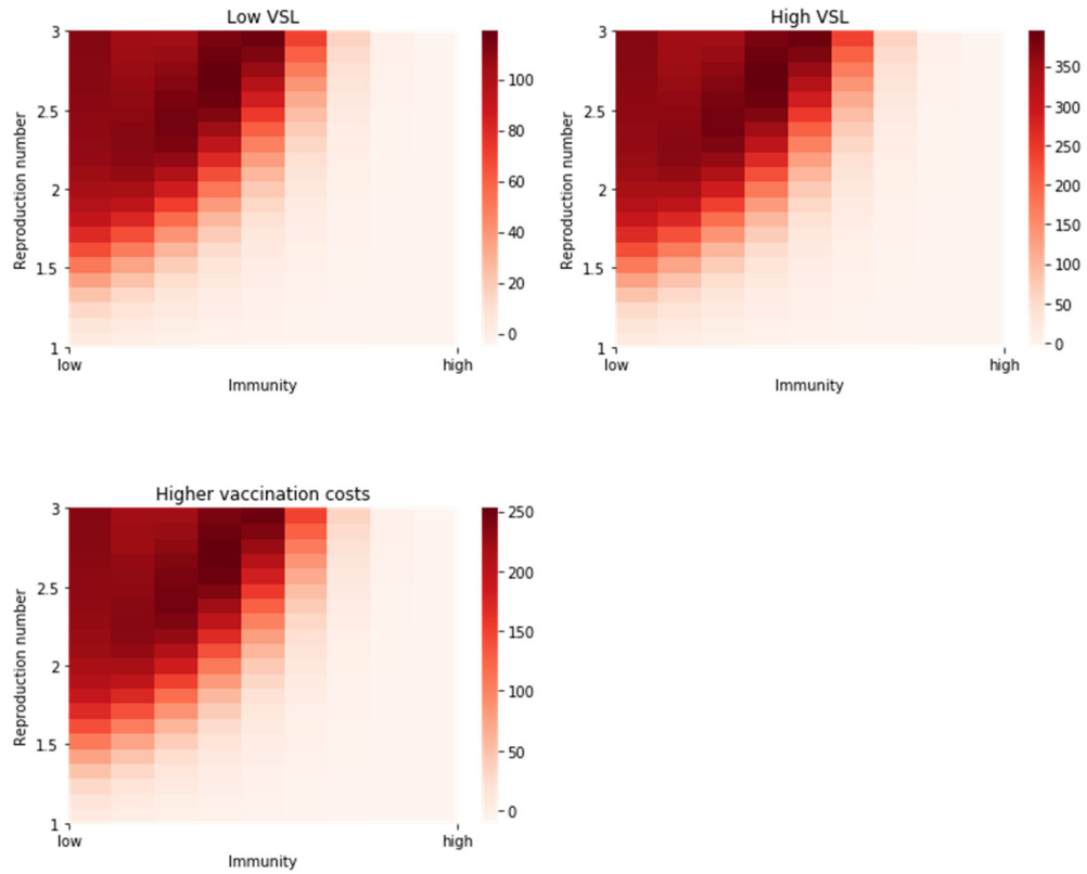
Figure B2. Sensitivity of net benefits to benefit and cost estimates as a function of the reproduction number (y-axis) and of the proportion of the population with infection-acquired or vaccination-acquired immunity (x-axis), various scenarios.
