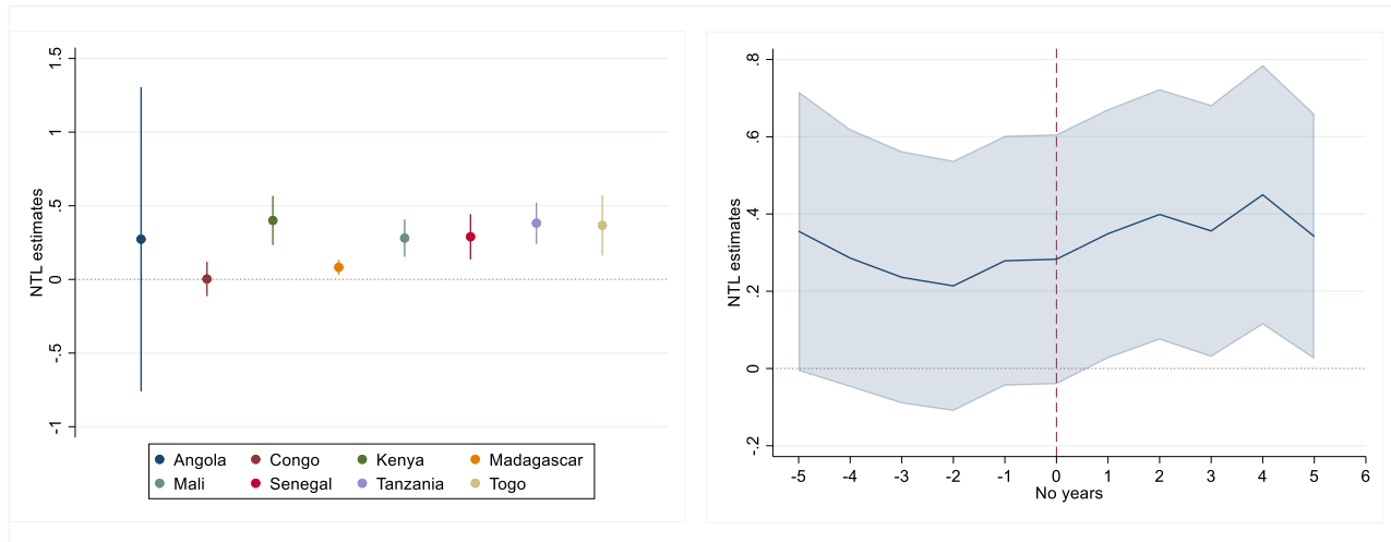
Figure 4. Effects of minigrid electrification on nighttime brightness across SSA and over time
