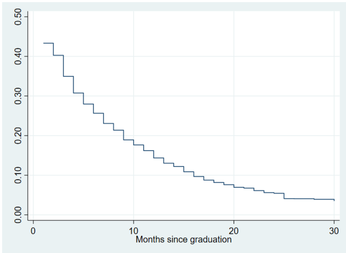
Figure A 1: Estimated Survivor Function
