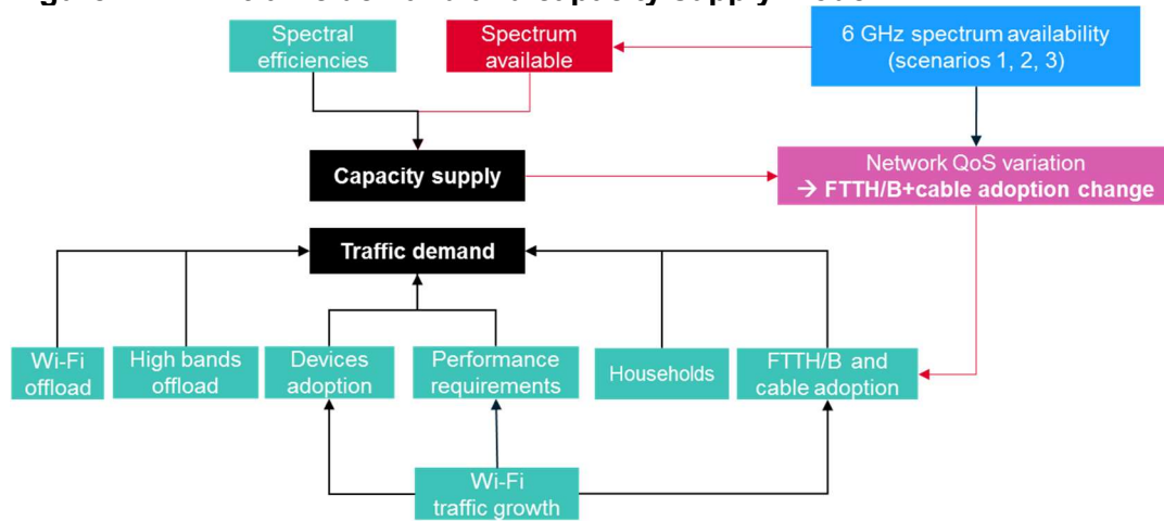
Figure 7: Wi-Fi traffic demand and capacity supply model
