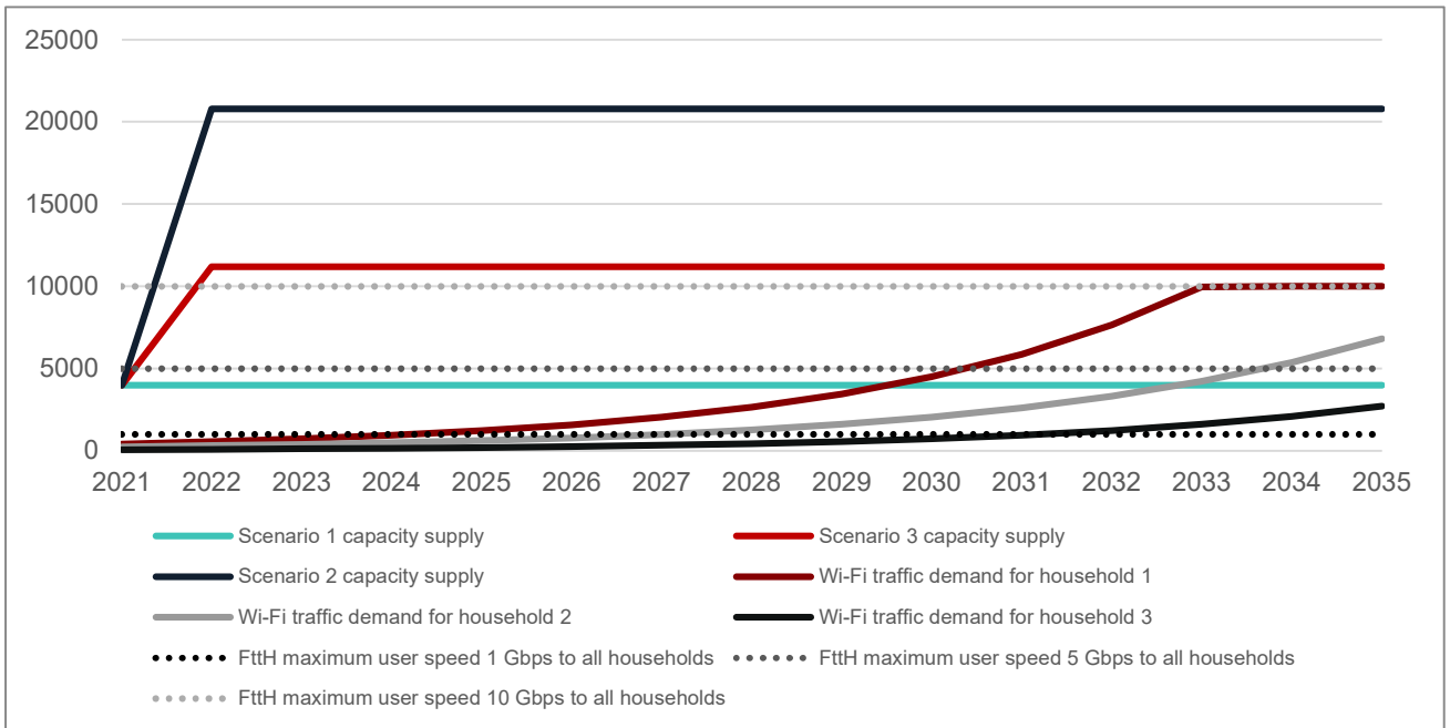
Figure 12a: Total Wi-Fi traffic demand and capacity supply (Mbps), with high bands utilised – house dwelling setting
