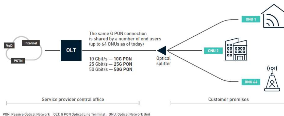
Figure 9: G-PON technology overview
