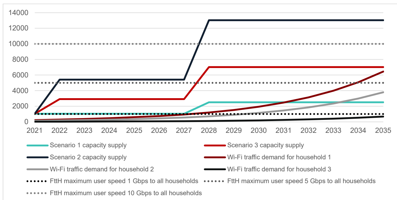
Figure 14B: Total Wi-Fi traffic demand and capacity supply (Mbps), with no high bands utilised – apartment setting
