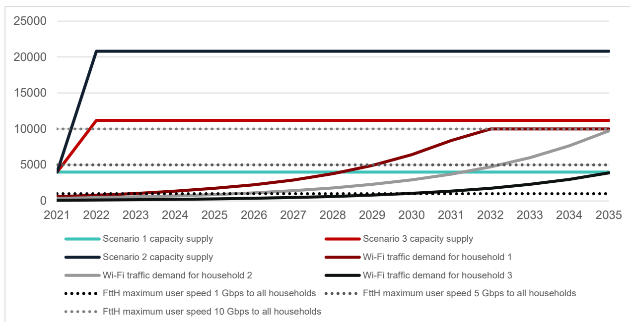
Figure 12b: Total Wi-Fi traffic demand and capacity supply (Mbps), with no high bands utilised – house dwelling setting
