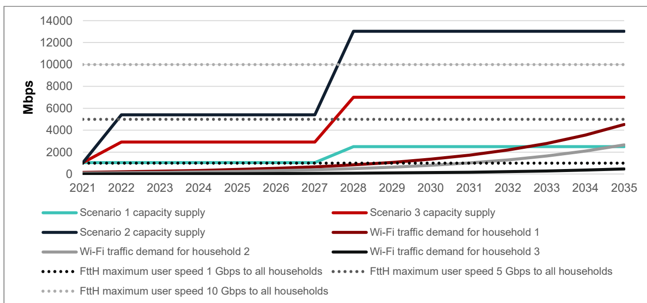
Figure 14A: Total Wi-Fi traffic demand and capacity supply (Mbps), with high bands utilised – apartment setting
