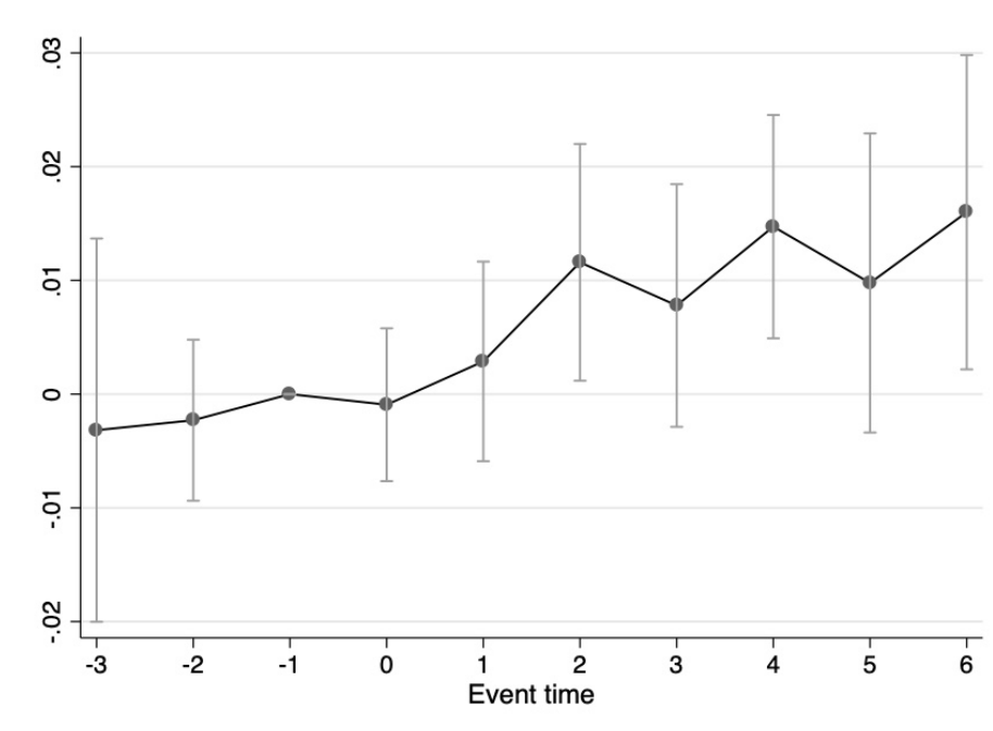
Figure 7: District-level event study
