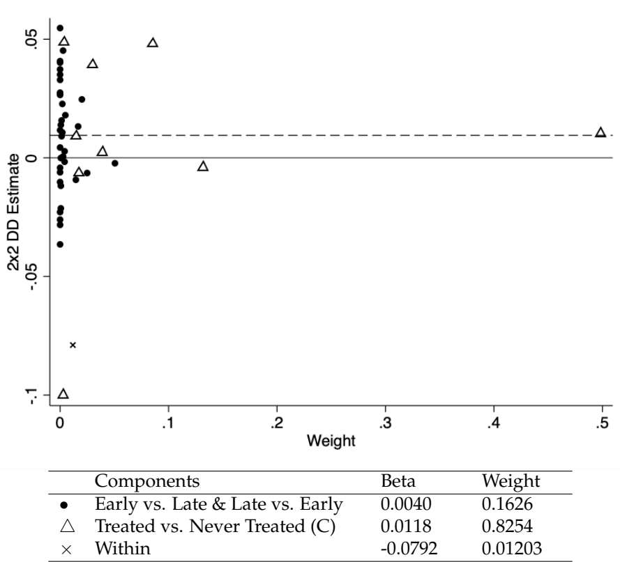
Figure 5: Bacon decomposition
