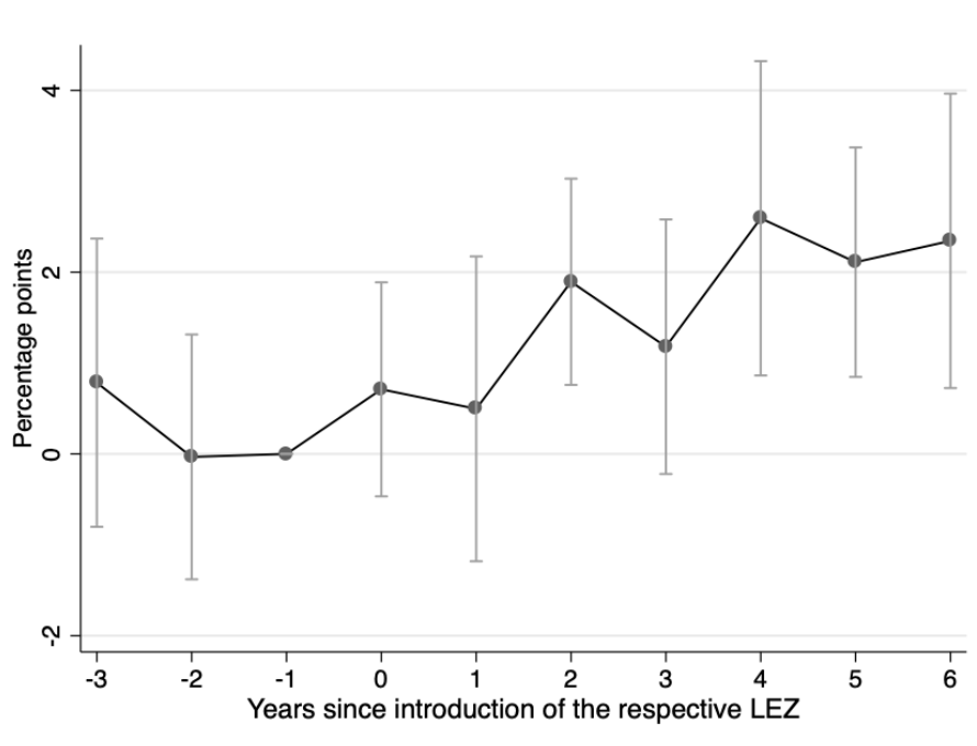
Figure 6: Event study of LEZs transition rates to the academic track
