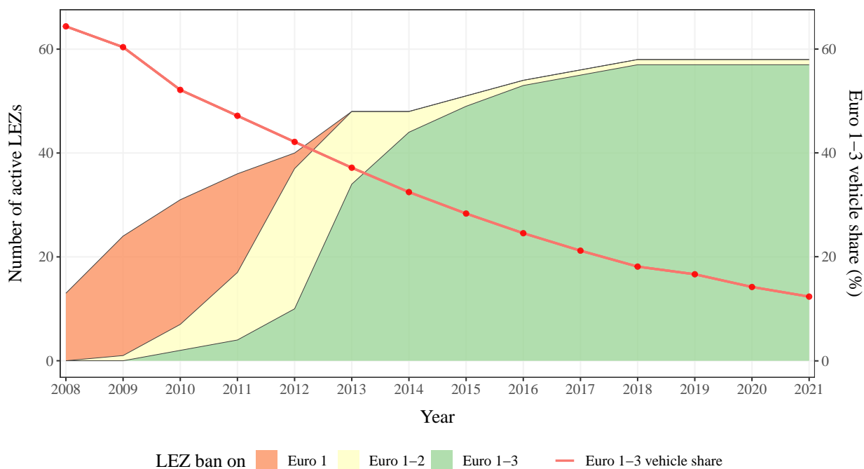
Figure 1: LEZs by emission standard in Germany over time
