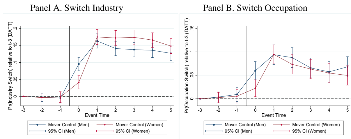
Figure 9: Switch Industry/Occupation
