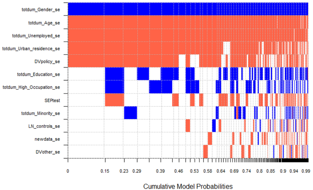
Figure 8: Model inclusion in Bayesian model averaging.
