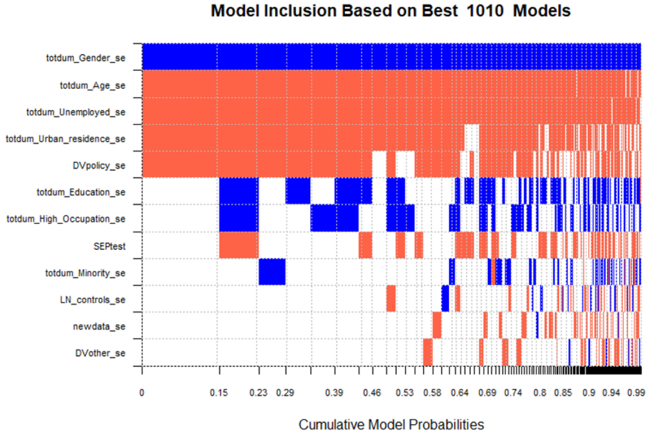
Figure 8: Model inclusion in Bayesian model averaging.
