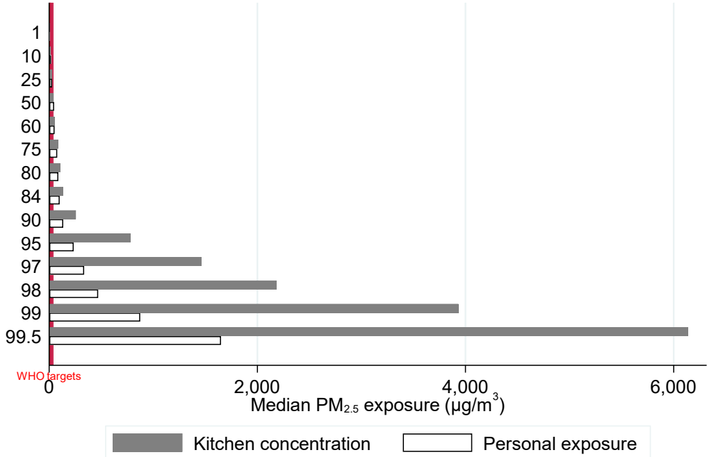
Figure B.1: Median kitchen concentration and personal exposure (PM 2.5 ), by percentiles
