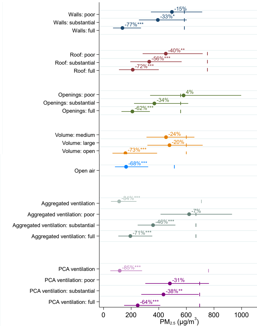
Figure 4: Associations between kitchen concentration and ventilation indicators
