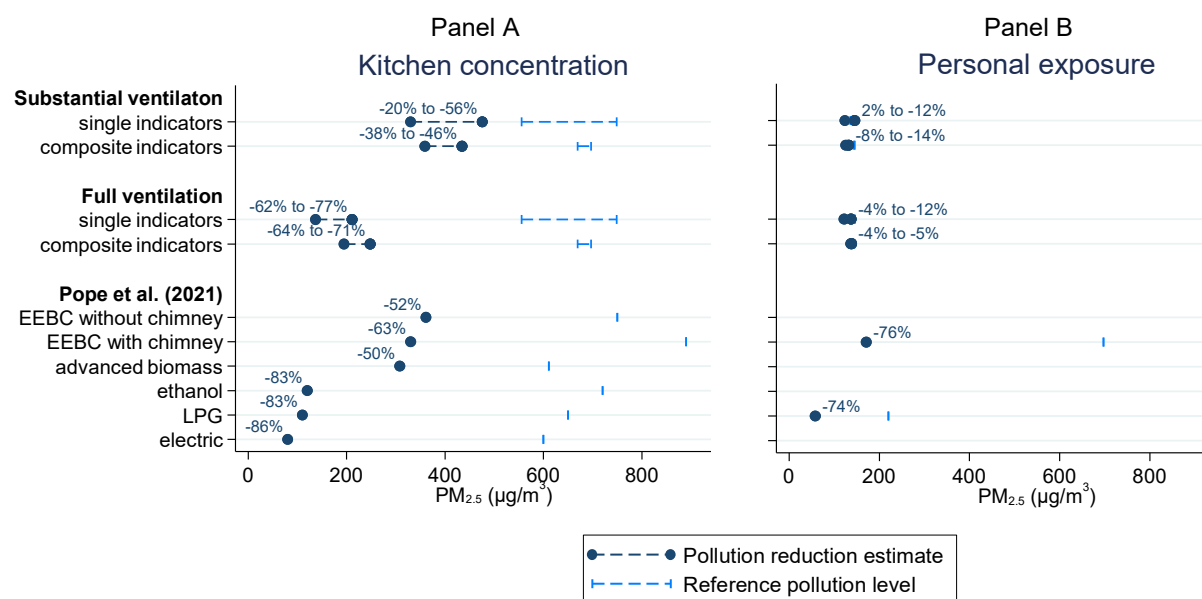
Figure 6: Reduction potentials compared to those from stove and fuel interventions
