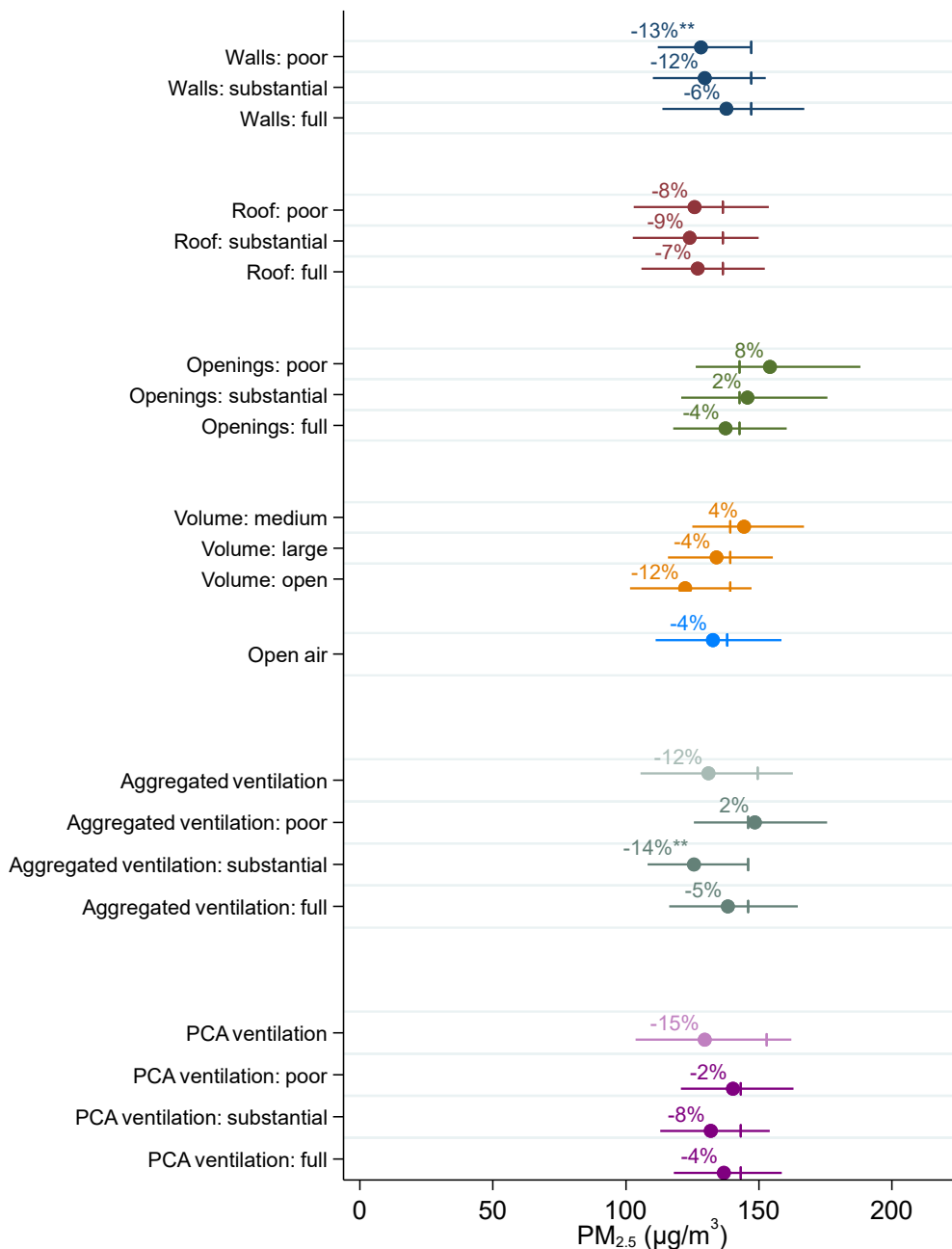
Figure 5: Associations between personal exposure and ventilation indicators
