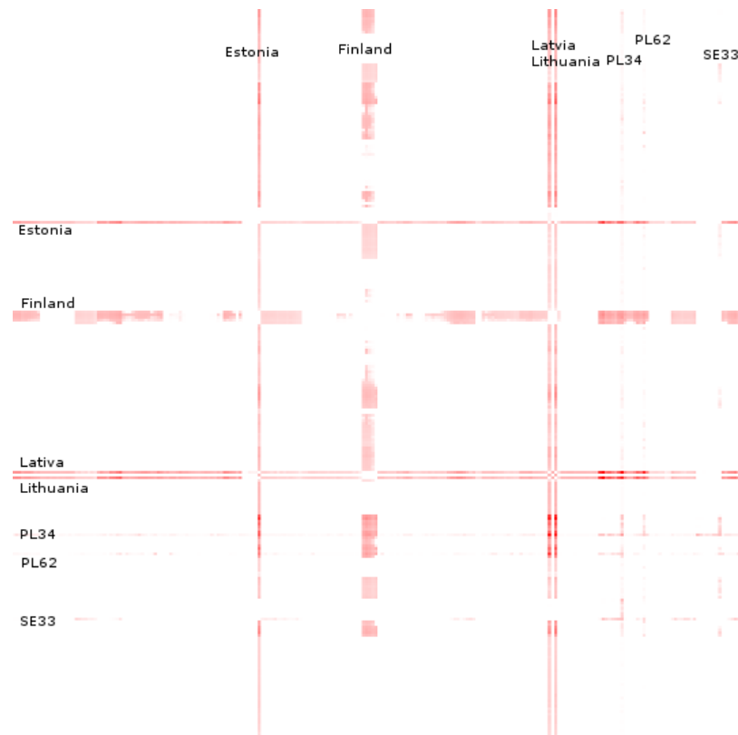
Figure 4 Heat map of the changes in transport costs due to investments in Podlaskie (PL34) in the north-east of Poland
