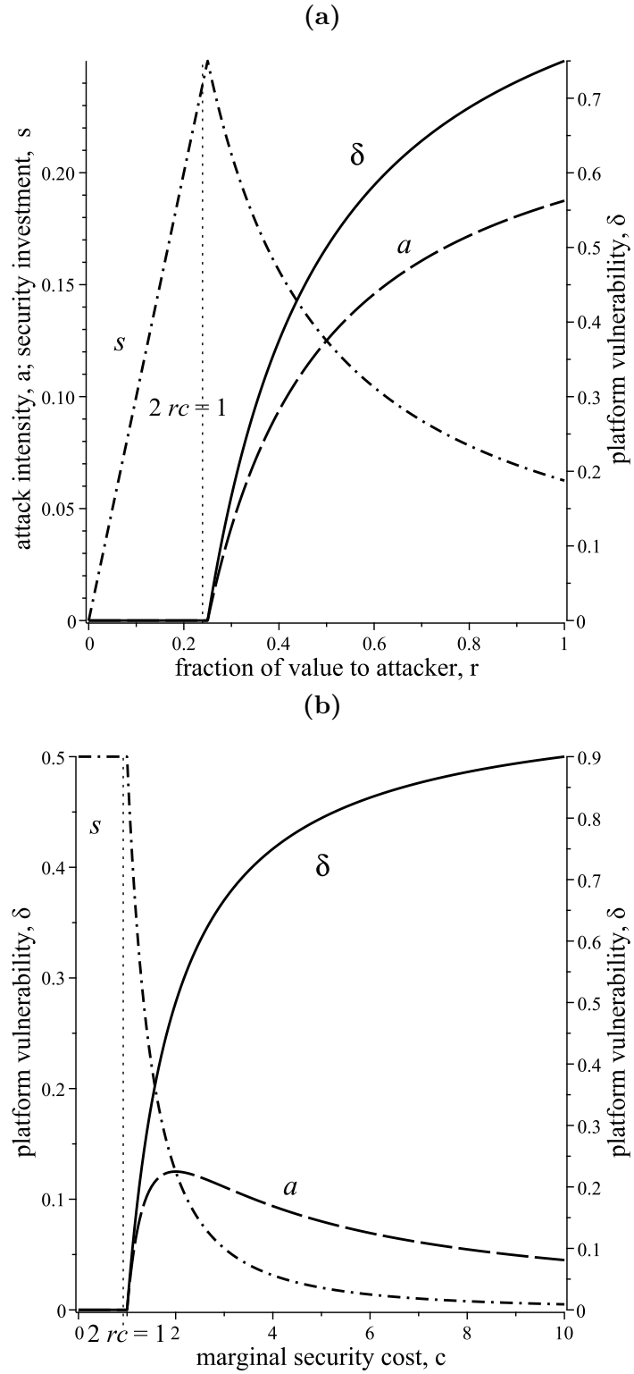
Figure 2: Comparative Statics
