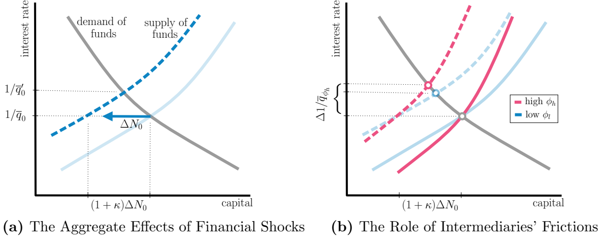
Figure A.1: The Aggregate Effects of Financial Shocks and the Degree of Intermediaries' Financial Frictions
