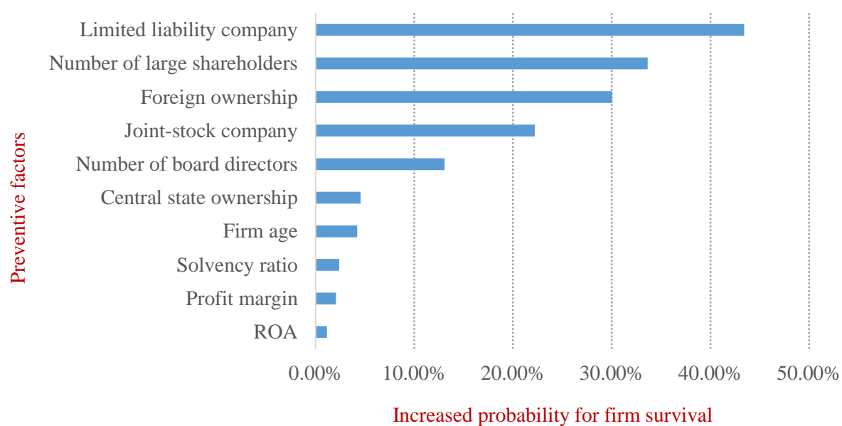
Figure 2: Average impact of selected covariates
