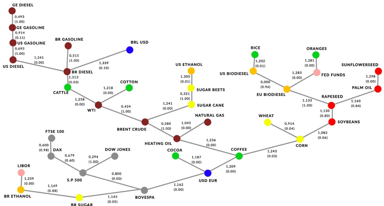
Figure 3: Minimum Spanning Tree - Period I
