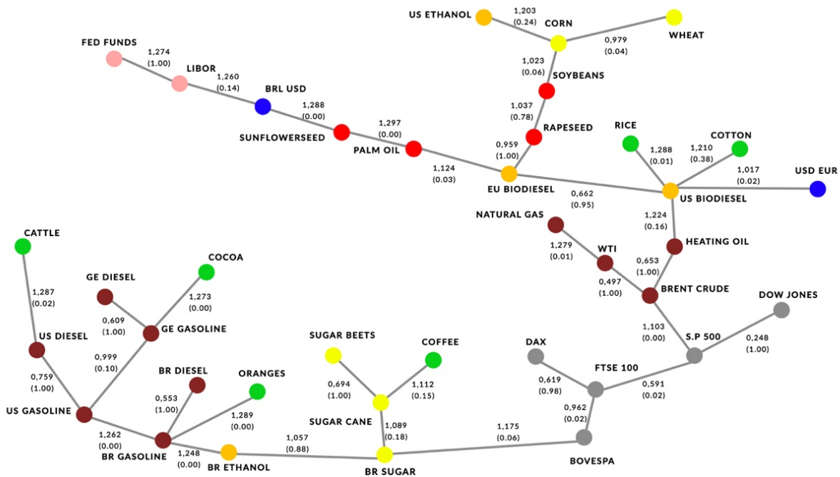
Figure 5: Minimum Spanning Tree - Period III
