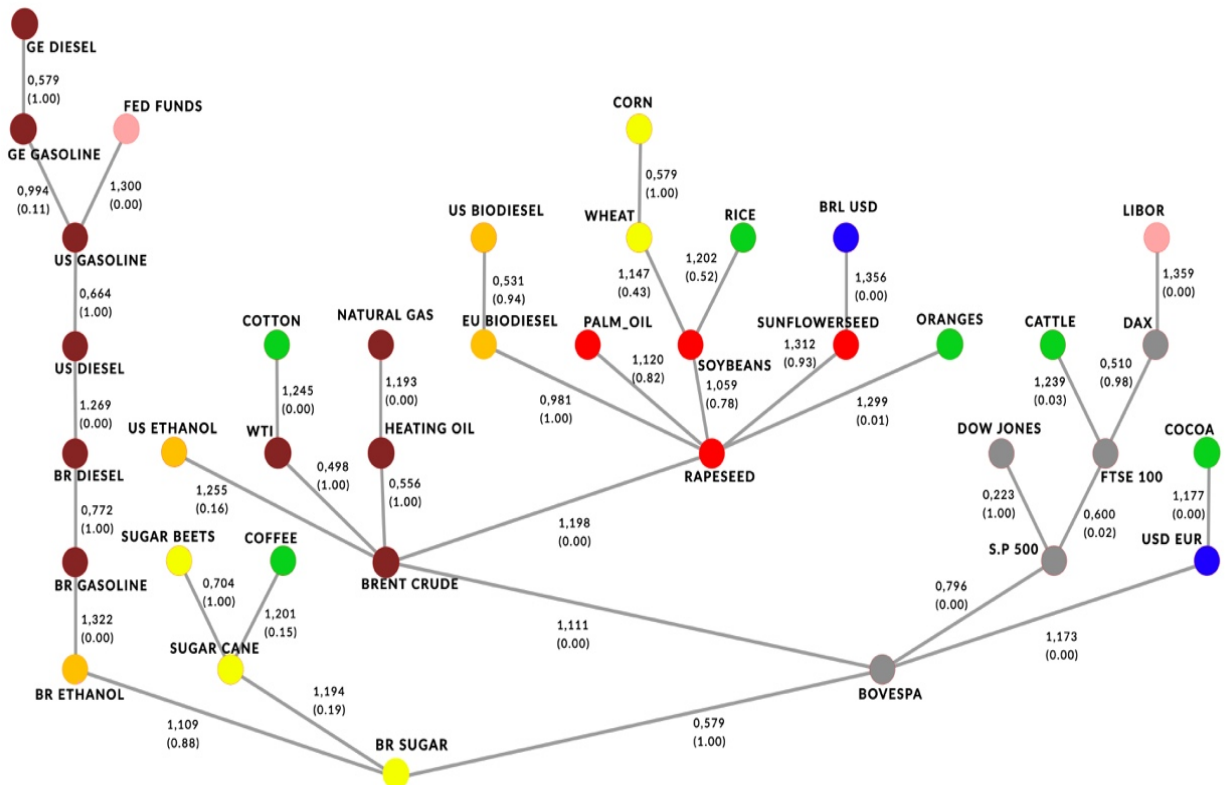
Figure 2: Minimum Spanning Tree – Entire period 2003-2020
