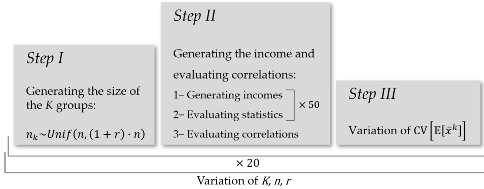
Figure 3: The Monte Carlo algorithm
