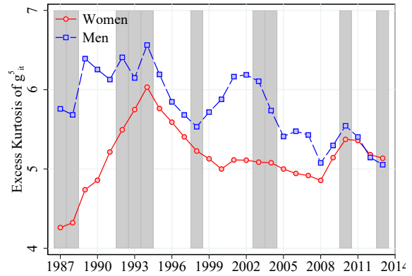
(b) Excess Crow-Siddiqui Kurtosis
