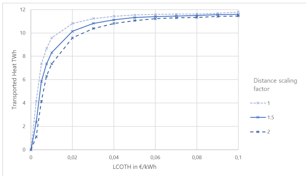
Figure 6: Sensitivity analysis of the transport distance
