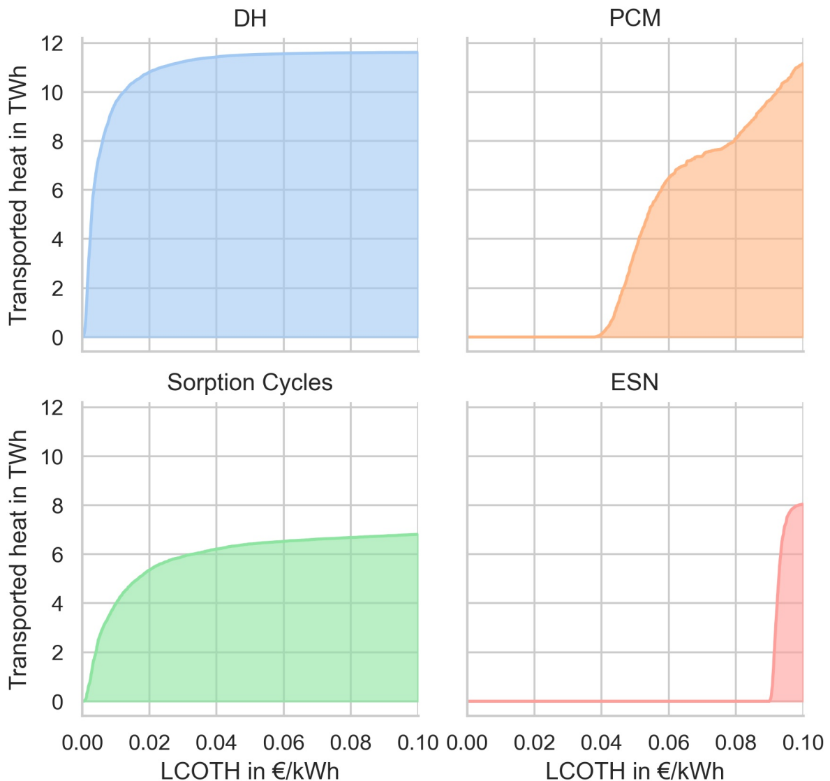
Figure 5: Cumulative LCOTH for cost optimisation for each technology
