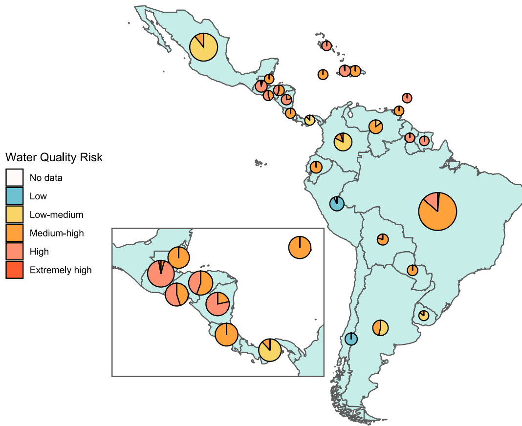
FIGURE 8: Population Proportion by Country That Lives Under Different Classifications of Quality-Based Physical Water Risk
