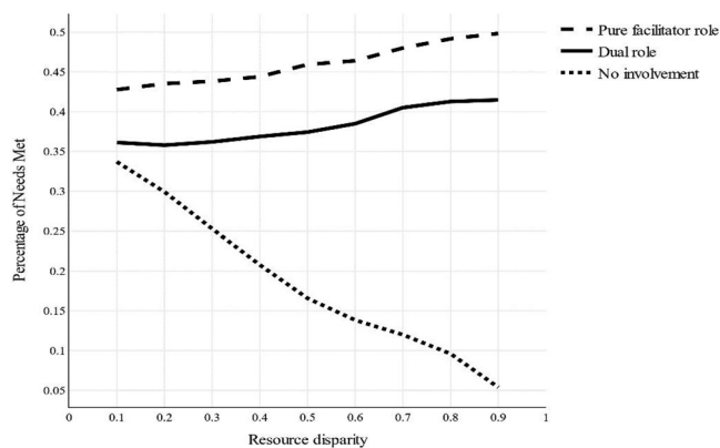
FIGURE 1 F Percentage of needs met as a function of resource disparity
