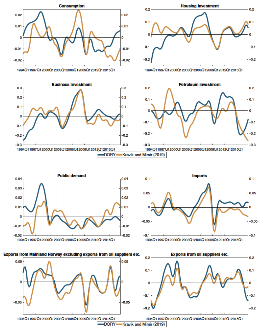
Figure 4: Estimated gaps. DORY and Kravik and Mimir (2019). Percent
