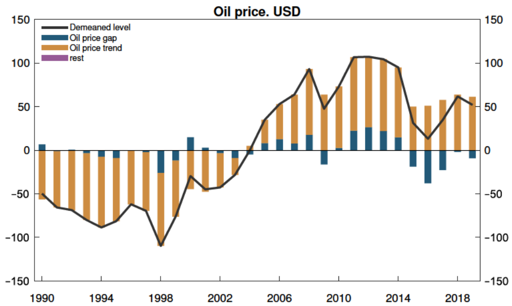
Figure 13: Decompositions of observables
