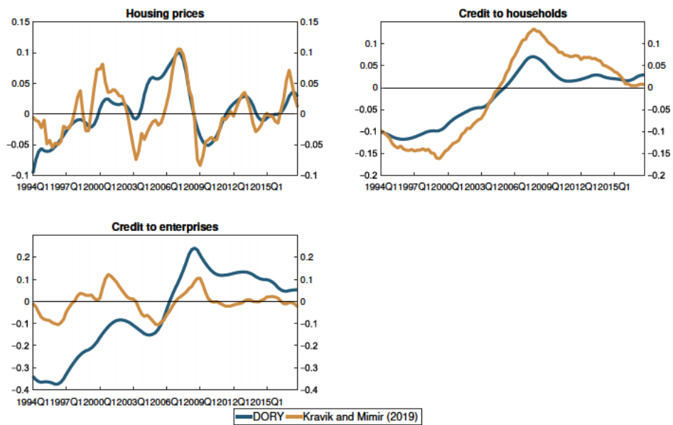
Figure 5: Estimated gaps. DORY and Kravik and Mimir (2019). Percent
