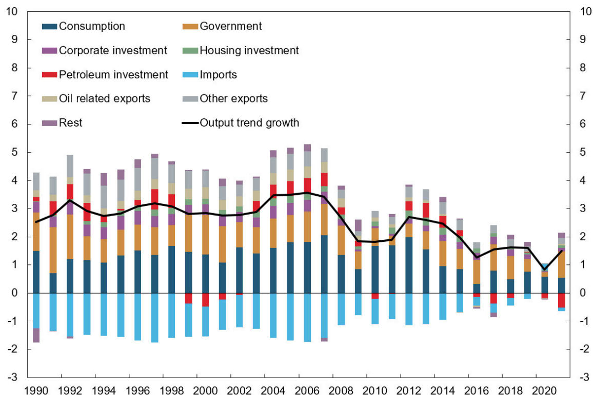
Figure 2: Decomposition of trend output growth. Percent
