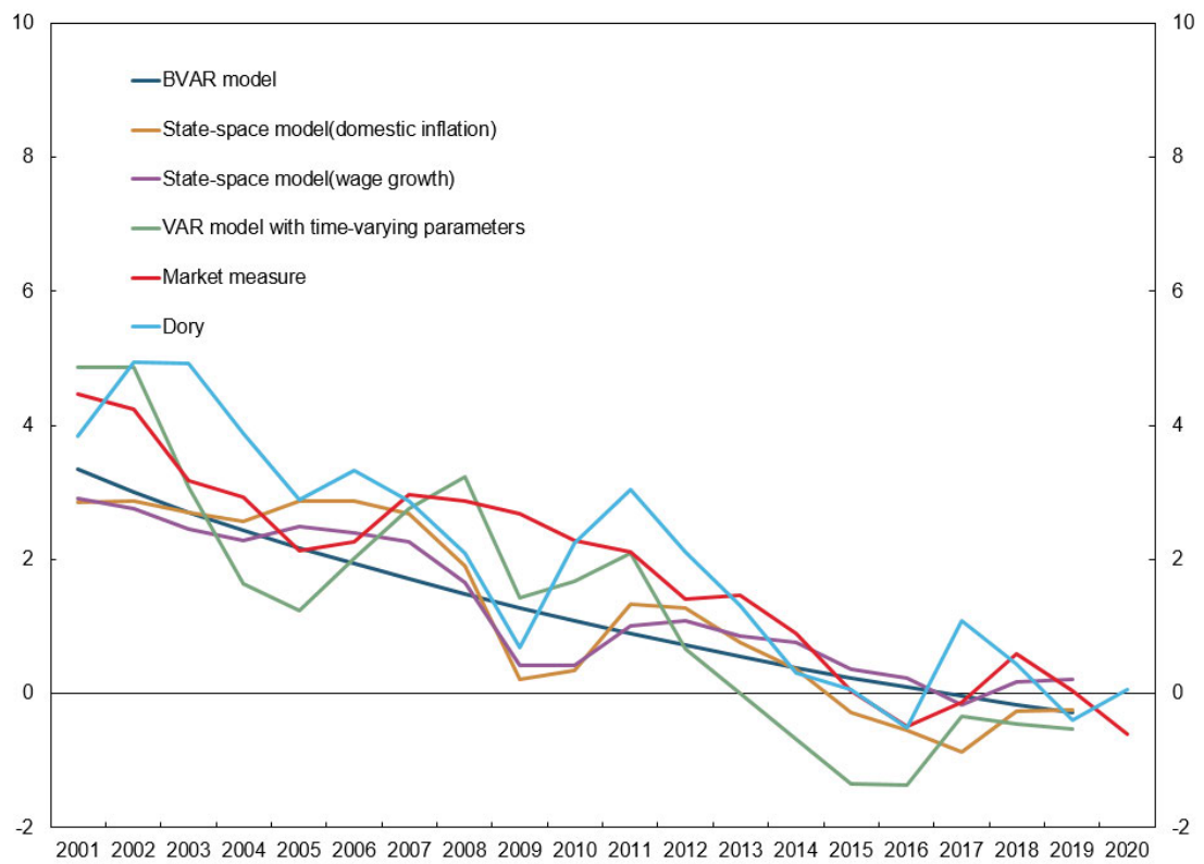
Figure 3: Estimates of the neutral real money market interest rate. Percent
