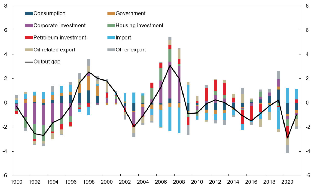
Figure 1: Decomposition of the output gap. Percent
