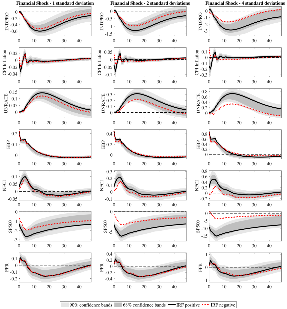
Figure 13: Impulse response functions of the VARX using g(u_{ft}) = u_{ft}^2 and leaving the impact response of INDPRO, CPI, UNRATE and EBP to the nonlinear term unrestricted. Black solid lines are the point estimates, the gray areas the 68% and 90% confidence bands of the bad financial shock. Red dotted lines are the point estimates of the good financial shock.
