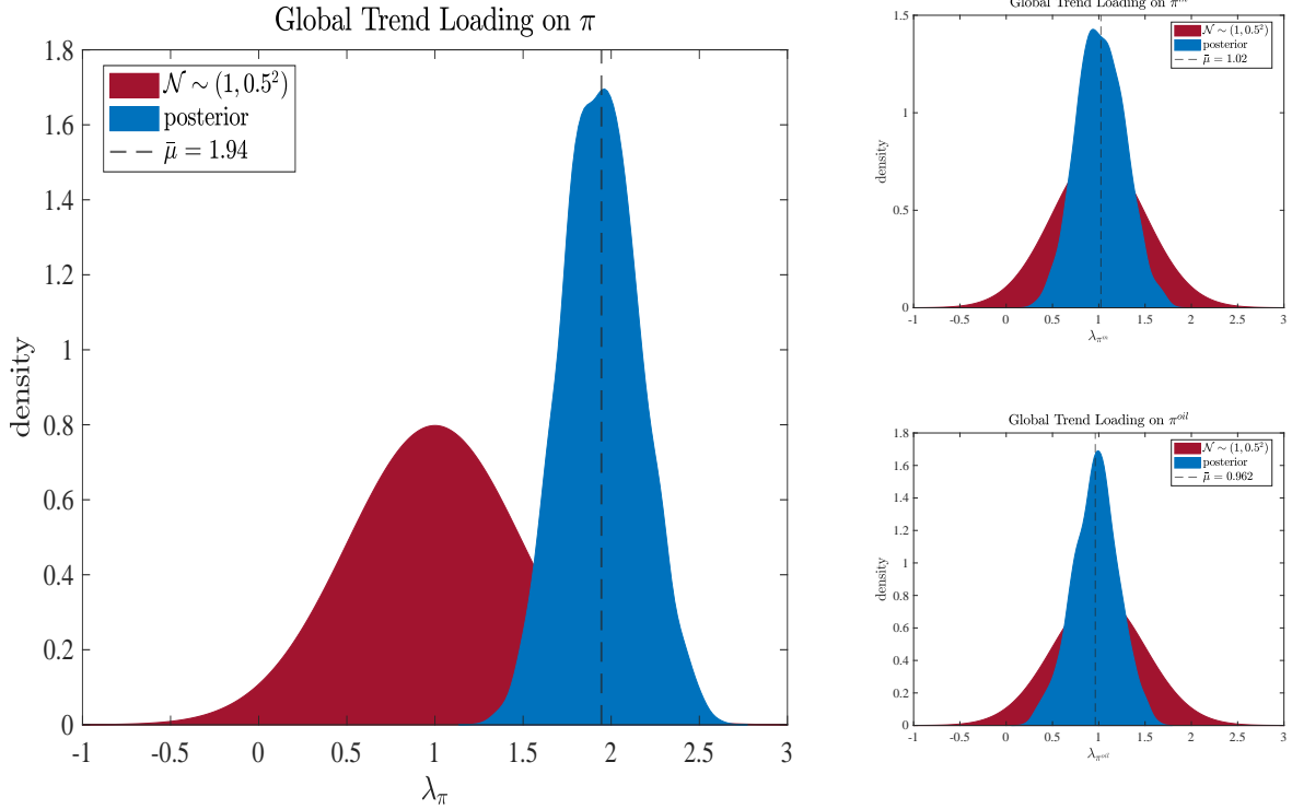
Figure 3: Prior and posterior distributions of the loadings
