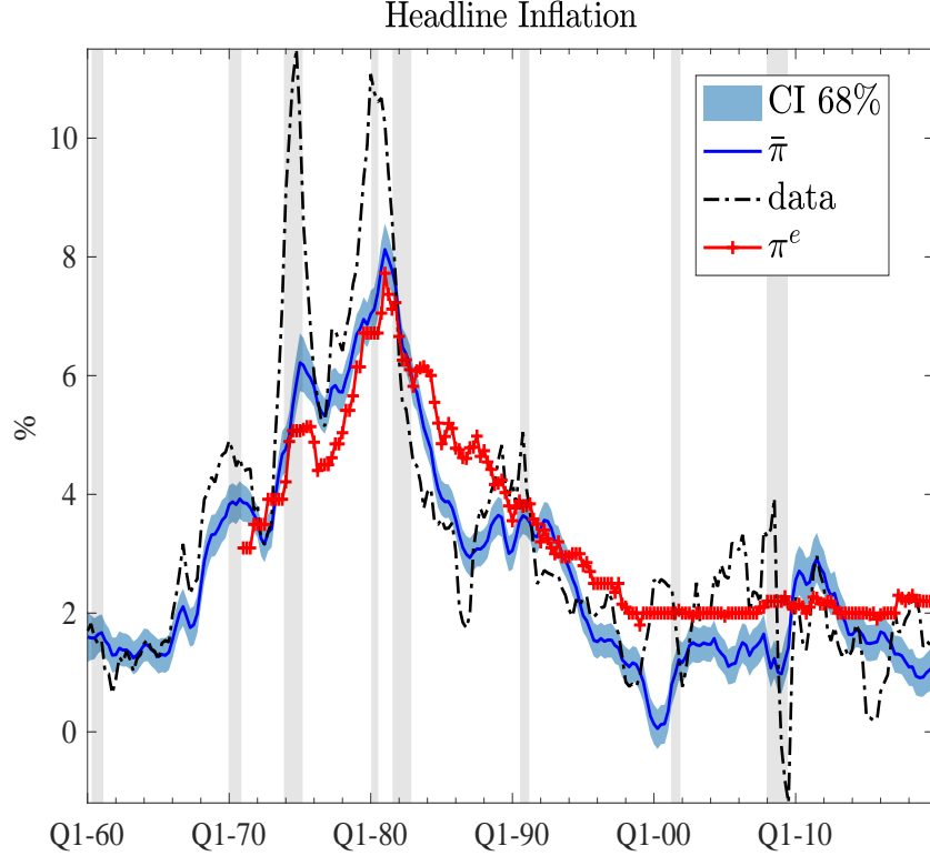
Figure 1: Trend inflation.
