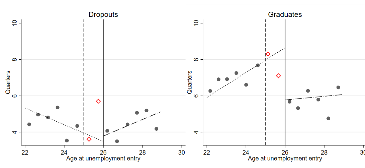
Figure A.23: Discontinuity at Age 26 of the Cumulative Number of Quarters in a Private Sector Job Paying More Than the Median Daily Wage, 7 Years After Entry Into Unemployment
