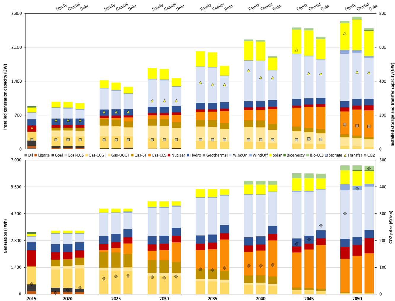
Figure 1: Impact of investment cost specifications on technology mix and CO 2 price
