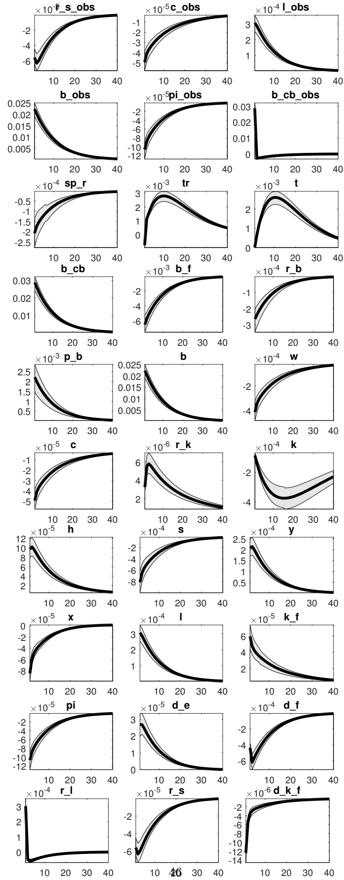
Figure 11: Bayesian IRFs QE Shock.
