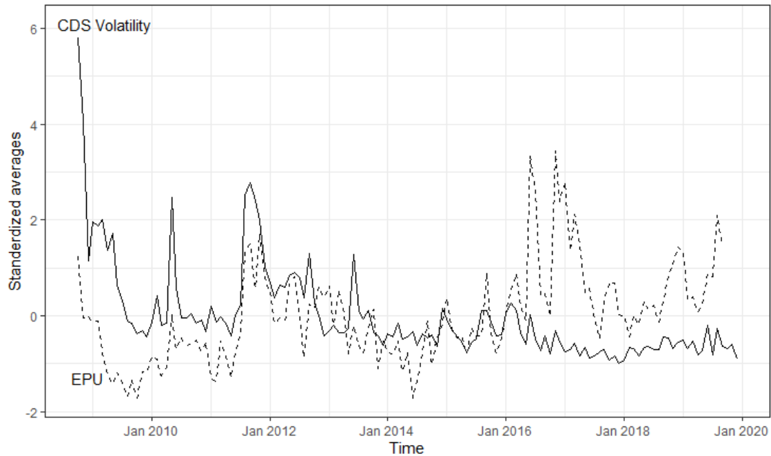
Figure 2: Standardized cross-sectional averages of CDS volatility and EPU indices over time.
