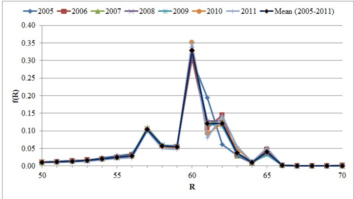
Figure A.1: The picture show the retirement probability for Austrian males in the years 2005 to 2011 (i.e. the values f(R, 2005 - R) , f(R, 2006 - R) , \dots , f(R, 2011 - R) ). The average retirement age over the years is given by 59.5 with a standard deviation (from 2005 to 2011) of 0.14. The standard deviation of the retirement ages (between 50 and 70) comes out as 2.98 with a standard deviation (from 2005 to 2011) of by 0.053.
