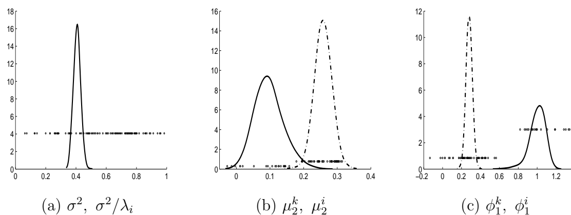
Figure 2: Series-specific heterogeneity. Group 1 (solid line), group 2 (dash-dotted).
