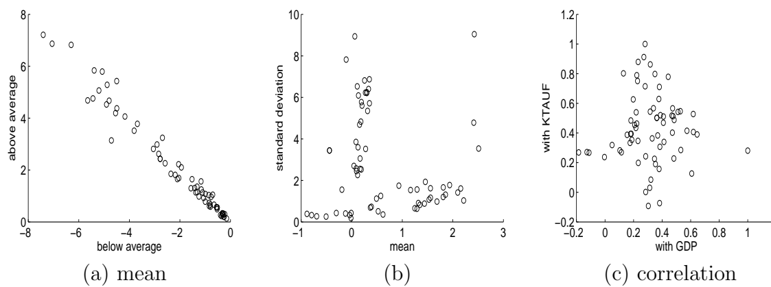
Figure 1: Data properties
