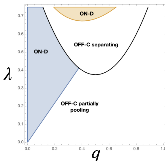
Figure 2: Equilibrium map in (\lambda, q) -space.
