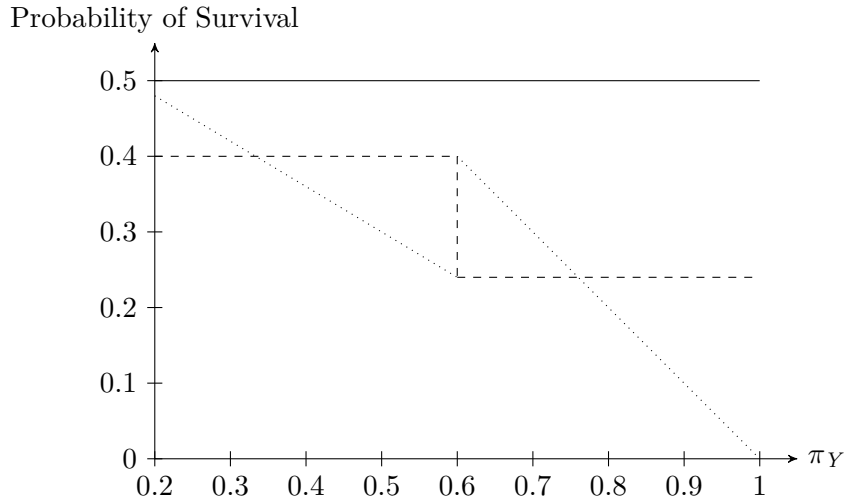
Figure 6: Buffoon Equilibria: Survival Probabilities as a Function of \pi_Y . Survival probabilities of X (dotted), Y (dashed) and Z (solid) as \pi_Y varies from 0.2 to 1, when \pi_X = 0.6 , \pi_Z = 0.4 , \beta_Z = 0.5 .
