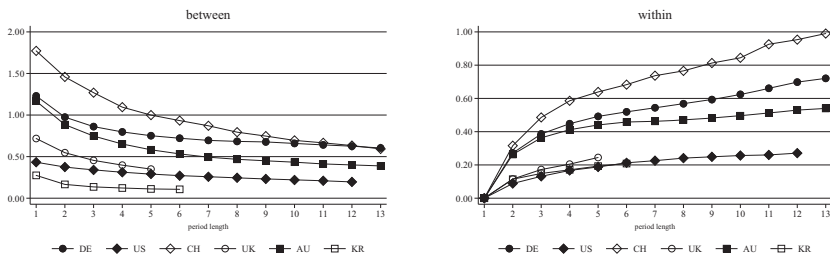
Fig. A2. MLD, government reduction of the between and within component by period length Source: Own calculations, CNEF.
