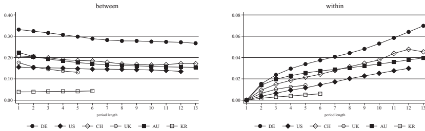
Fig. 2. Government reduction of the Theil between- and within-group component by period length
