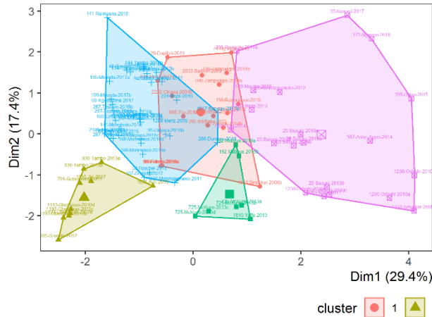
(a) Cluster plot by first principal components
