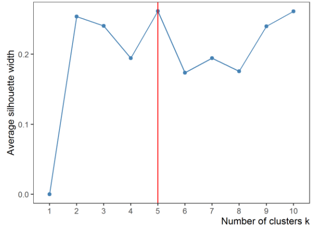
(b) Average silhouette width by number of clusters
