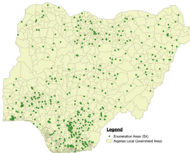
Figure 3: EAs of waves 2010/11, 2012/13, and 2015/16 in Nigeria
