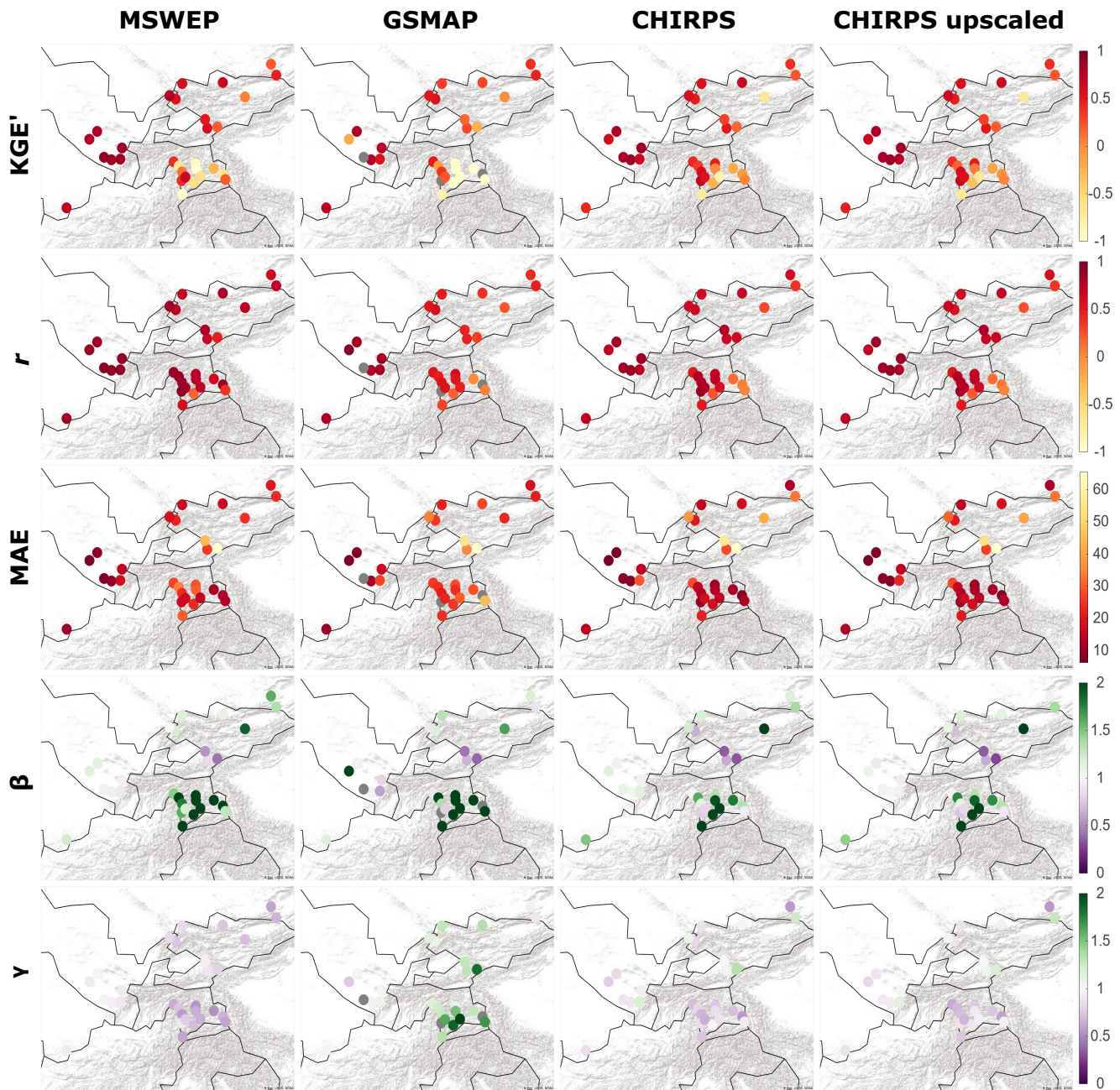
FIGURE 4 KGE', its components ( r , \beta , \gamma ), and MAE derived from a monthly timescale. The colours for KGE', r , and MAE range from light yellow (very poor performance) to dark red (best performance). For \beta and \gamma , white colours represent their best performance, while underestimation is depicted in dark purple and overestimation is depicted in dark green. Grey colour identifies stations not available for product evaluation (i.e., GSMAP, data before 2000). The black outlines correspond to the countries (see Figure 1 for a detailed map of the region) [Colour figure can be viewed at wileyonlinelibrary.com ]
