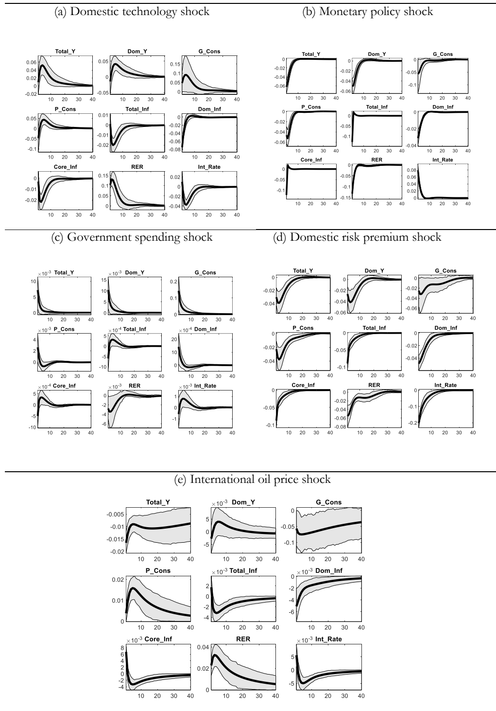
Figure 3: Bayesian impulse responses to selected structural shocks
