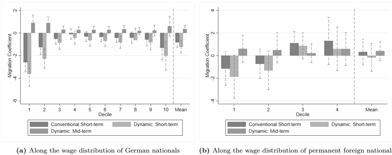
Figure 7: Panel (a) shows the estimated immigration coefficients on wages along the German nationals' wage distribution with 90% confidence intervals. Panel (b) shows the estimated immigration coefficients on wages along the wage distribution of permanent foreign nationals with 90% confidence intervals.
