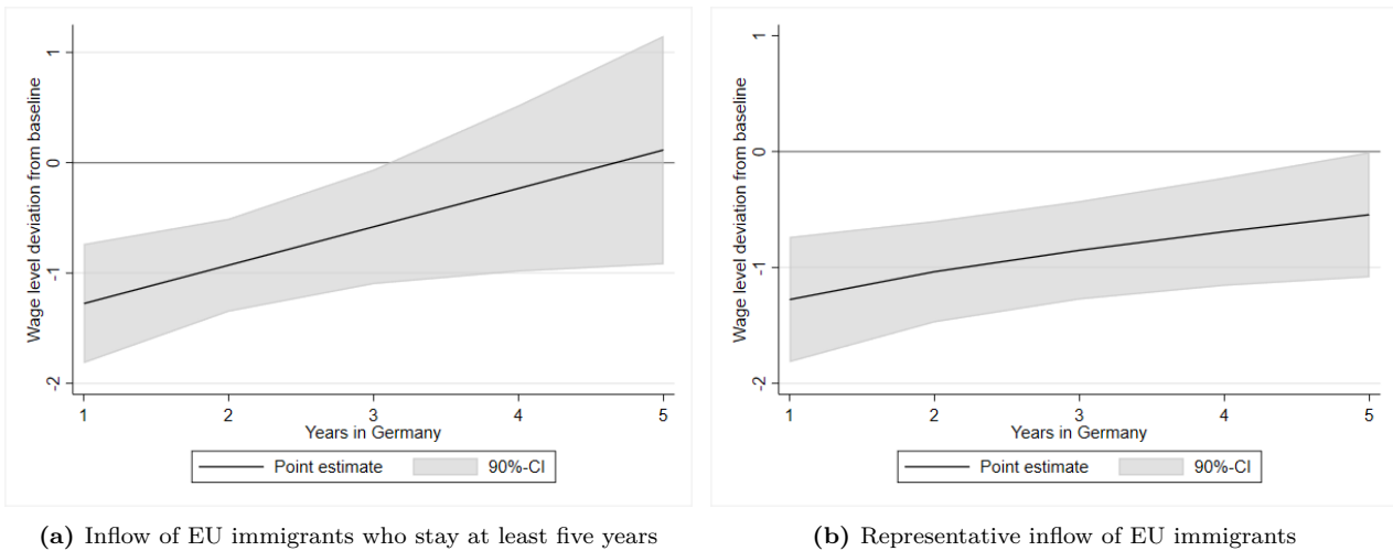
Figure 8: Panel (a) illustrates the dynamic impact of a one percent inflow of EU immigrants who stay at least five years in Germany on the level of mean wages of German nationals relative to the zero immigration baseline scenario in percent. Panel (b) illustrates the dynamic impact of a representative one percent inflow of EU immigrants, i.e. here we account for the fact that year-by-year a certain fraction leaves Germany again (in line with the survival rates estimated above), on mean wages of German nationals relative to the zero immigration scenario in percent. Confidence intervals are based on Wald tests.
