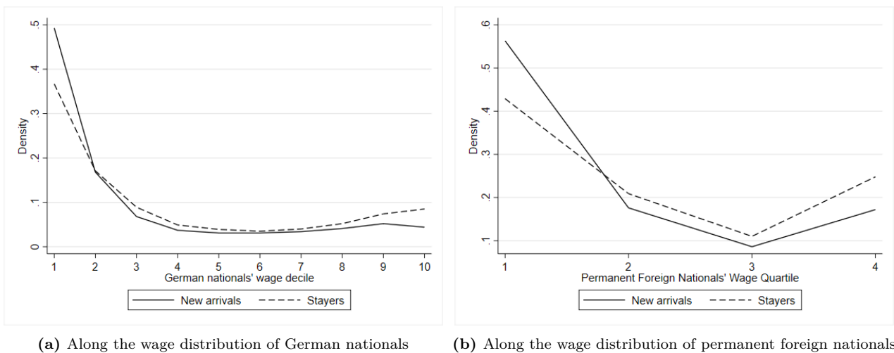
Figure 11: Panel (a) shows the densities of new arrivals and stayers, respectively, in each decile of the regional wage distribution of German nationals; i.e., the share earning a wage within decile x \in [1, 10] of the wage distribution of German nationals. Panel (b) shows the corresponding densities in each quartile of the permanent foreign nationals' regional wage distribution.
