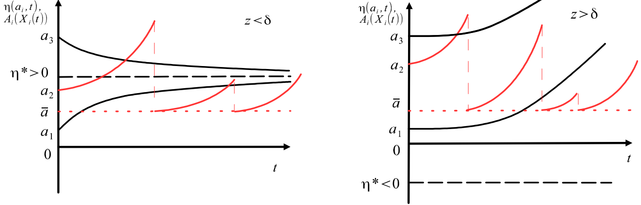
Figure 5 Realized wealth paths (red) vs. expected wealth paths (black) of a dynasty
