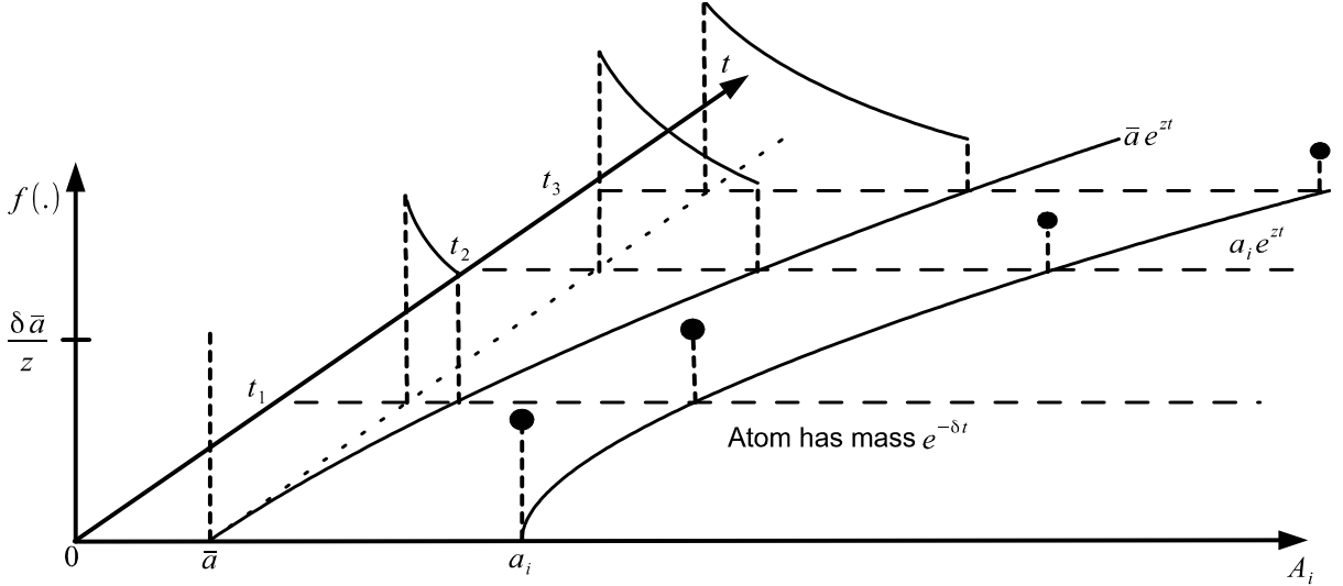
Figure 6 Dynamics of the wealth density for an initially degenerate distribution
