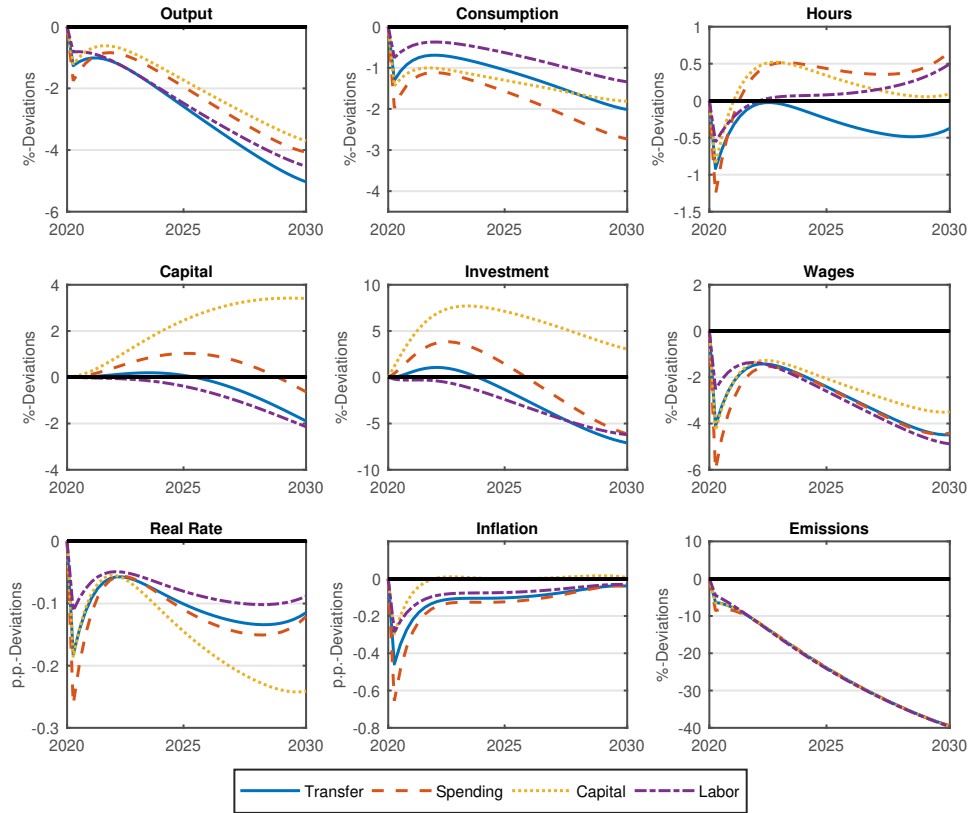
Figure E.1: Transition dynamics of the main variables between 2020–2030 (with output gap target)
