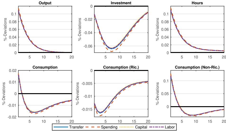
Figure 1: IRFs to a Government Spending Shock
