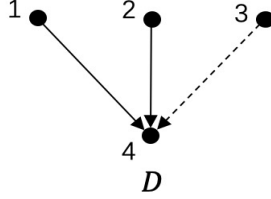
Figure 3: The digraph of Example 3.3.
