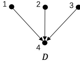
Figure 1: The digraph of Example 3.1.
