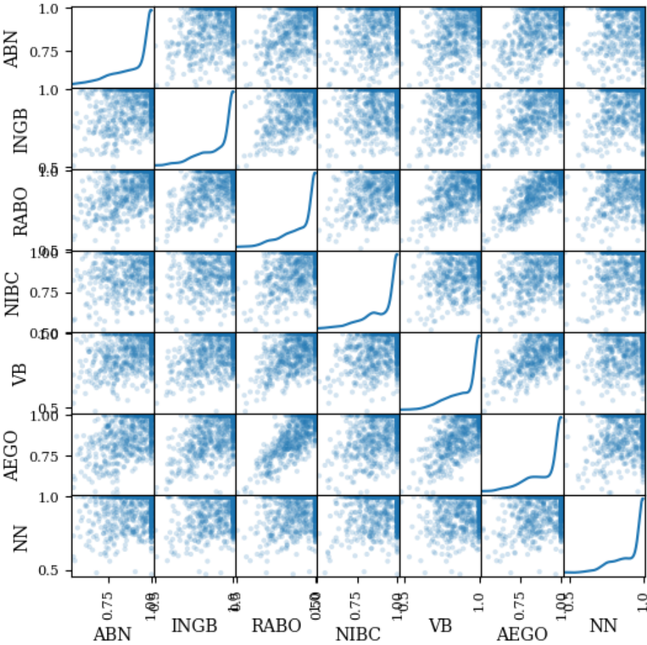
Figure 18: Recovery Rate Simulations
