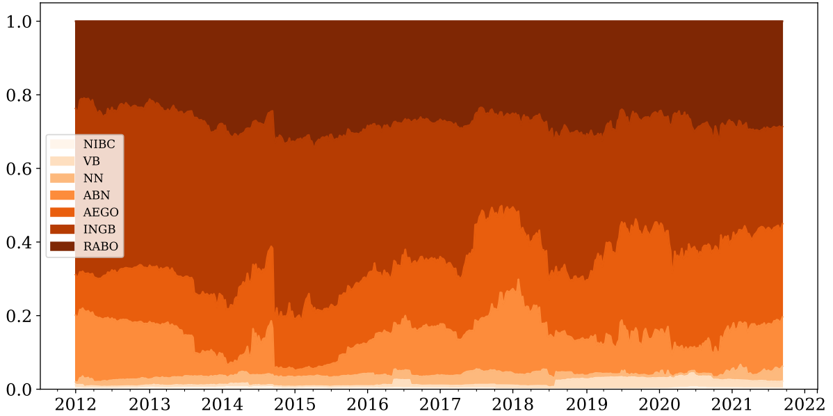
Figure 9: 99% MES (Percentage Contribution)
