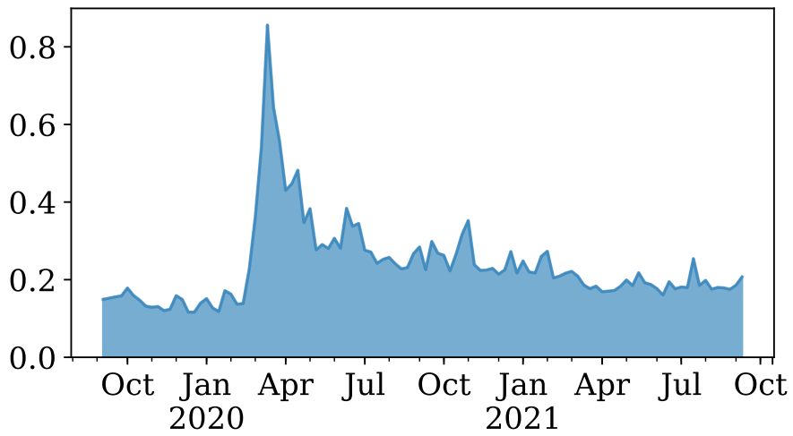
Figure 14: VSTOXX
