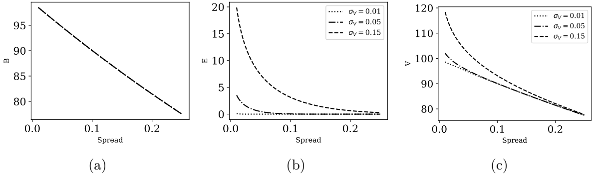
Figure 11: Merton Model
