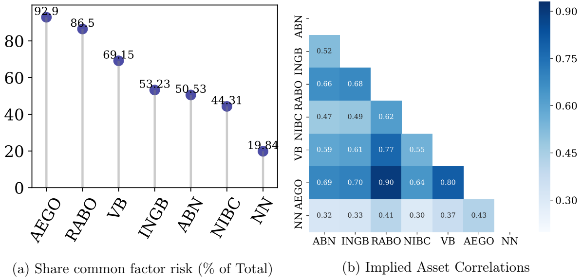
Figure 2: Common Factor Loadings
