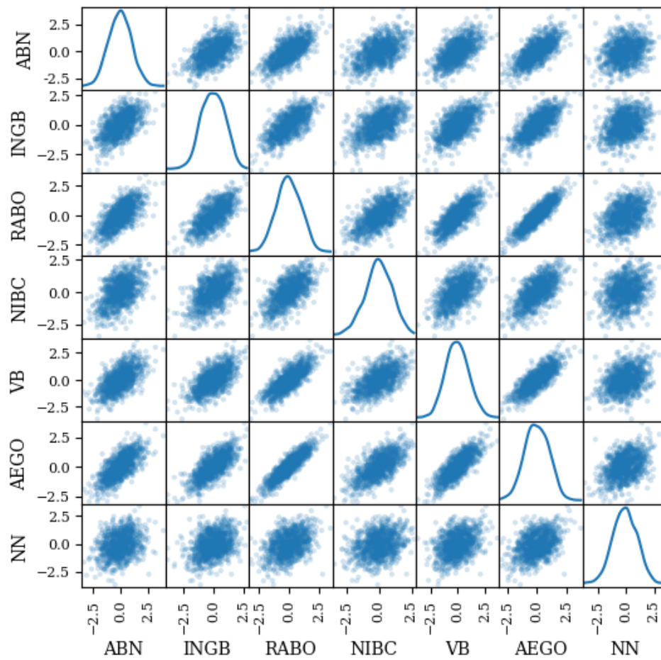
Figure 17: Asset Simulation
