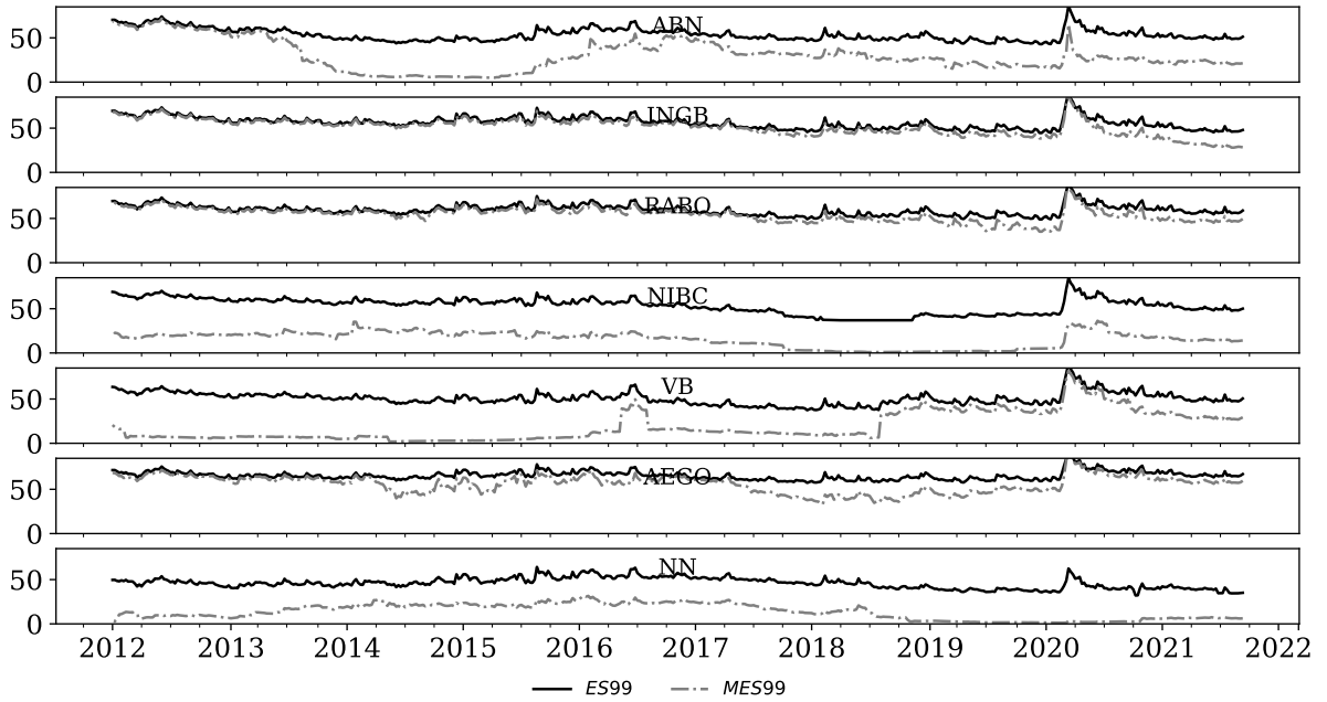
Figure 8: Backtest, 99% MES
