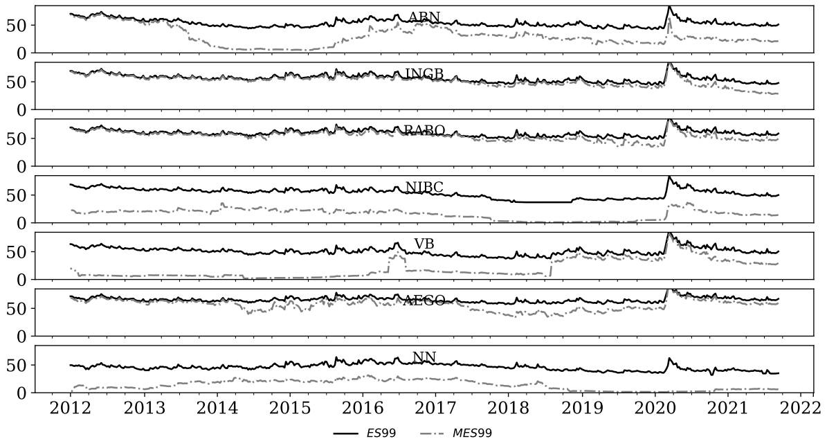
Figure 8: Backtest, 99% MES
