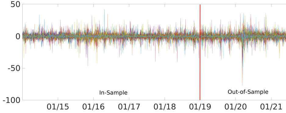
Figure 2: Daily (%) log-returns for 496 individual stock components of the S&P500 over the sample January 2, 2014 to June 30, 2021. The red line on January 2, 2019 indicates the beginning of out-of-sample period.
