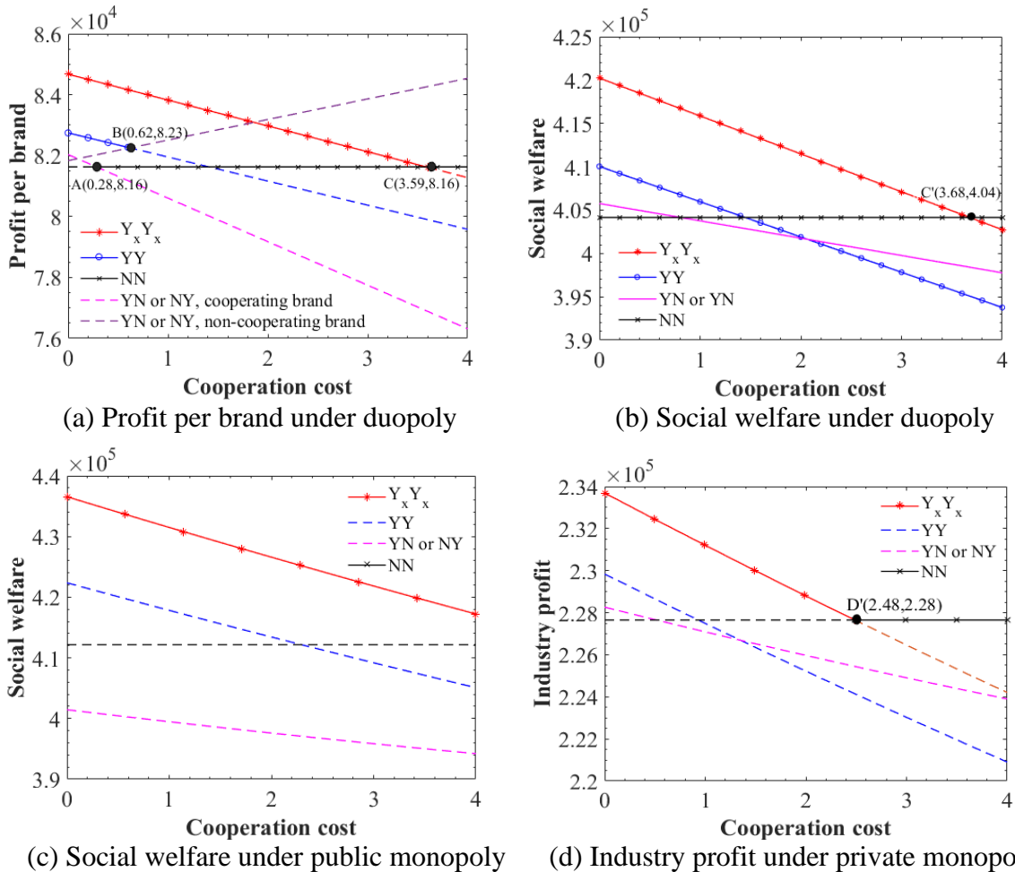
Fig. 5. Effects of cooperation cost on the profit and social welfare.
