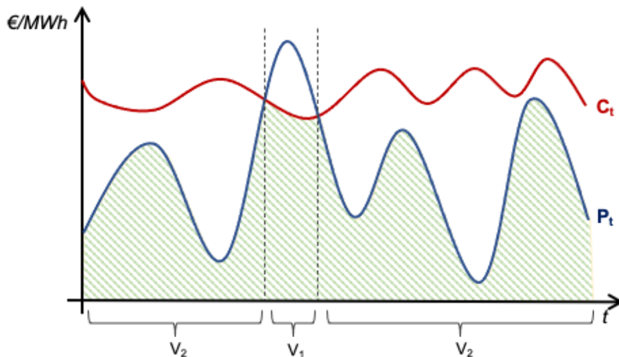
Figure 1: The green area represent the operating profits for a firm capacity supplied by a VRE under the existence of the CRM. The x-axis corresponds to time t , the y-axis are revenues, measured in Euro/MWh. The red line represents the marginal costs of the marginal technology, C_t ; the blue line represents the day-ahead electricity prices P_t . The vertical dashed lines identify the regimes of the value function, as described by equation (6).
