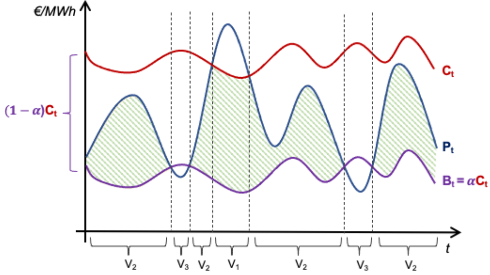
Figure 2: The green area represent the operating profits for a firm capacity supplied by a CCGT power plant under the existence of the CRM. The x-axis corresponds to time t , the y-axis are Euro/MWh. The red line represents the marginal costs of the marginal technology, C_t ; the blue line represents the day-ahead electricity prices P_t ; the cost of generating power from the CCGT is given by the purple curve \alpha C_t . The vertical dashed lines identify the regimes of the value function, as described by equation (14).
