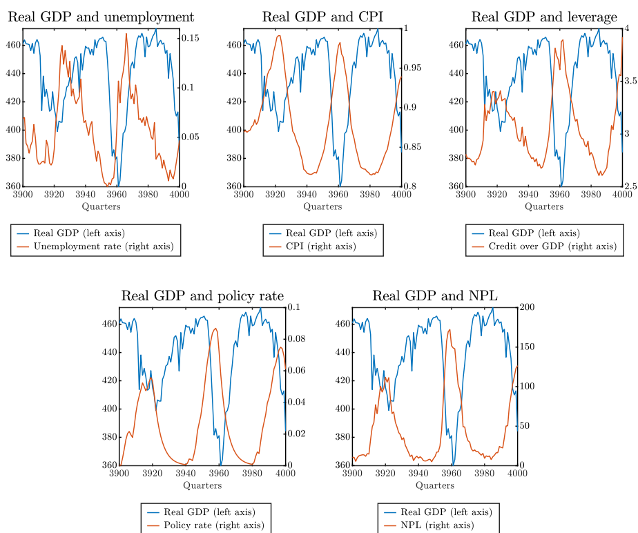
Figure 7: Endogenous business cycle.
