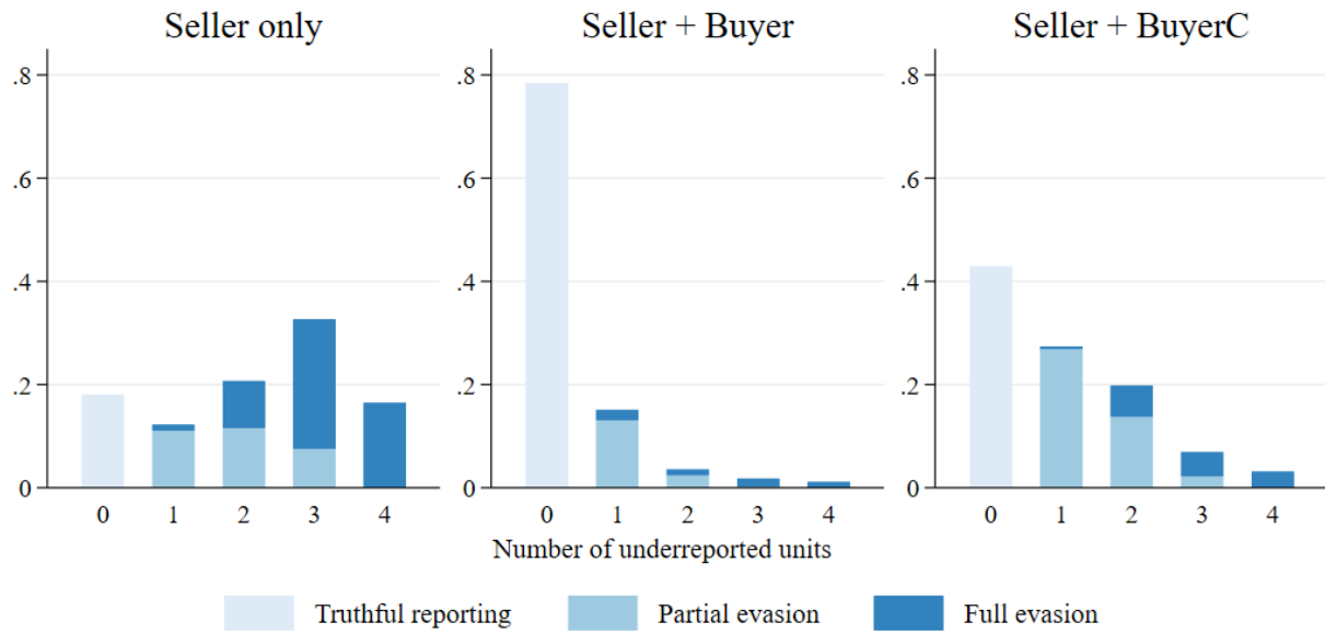
Figure 3. Under-reporting
