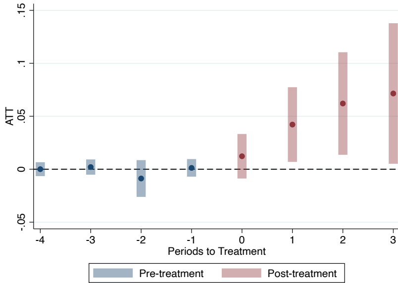
Figure 1: Staggered DID
