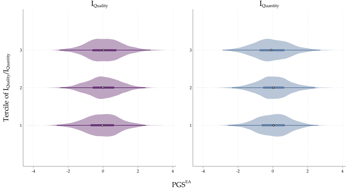
FIGURE 3 – \text{PGS}^{\text{EA}} Distribution by \text{I}_{\text{Quality}} and \text{I}_{\text{Quantity}}
